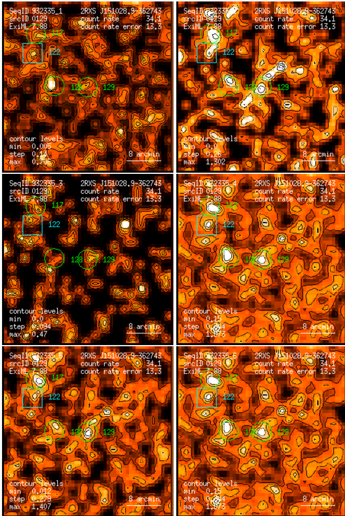
Figure 129: RASS 932335: detection 0129: band rate images, Gaussian filter: (1) PSPC channels 11 – 41, (2) 52 – 90, (3) 91 – 201, (4) 11 – 235, (5) 52 – 201, (6) 11 – 201. Broad band rates in counts/ks. Band rate contour levels in counts/ks/arcmin 2 .
