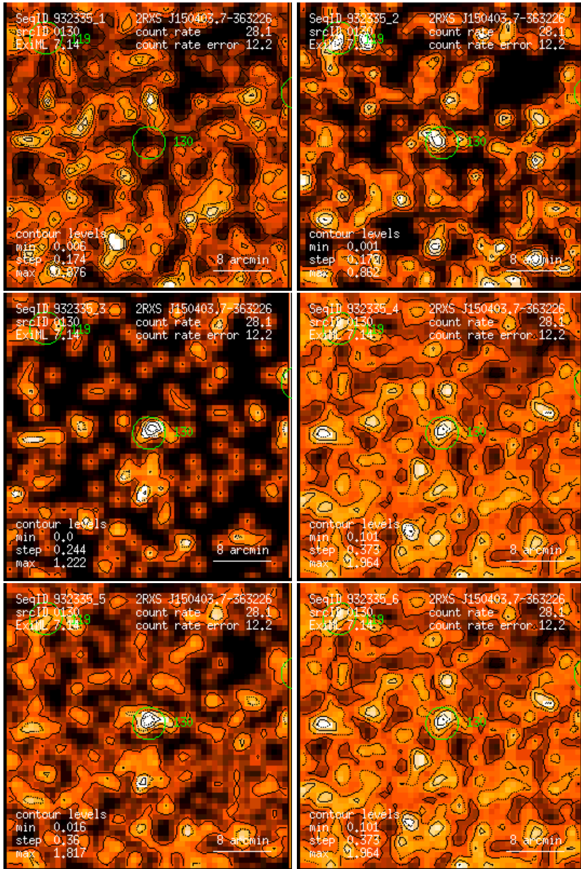
Figure 130: RASS 932335: detection 0130: band rate images, Gaussian filter: (1) PSPC channels 11 – 41, (2) 52 – 90, (3) 91 – 201, (4) 11 – 235, (5) 52 – 201, (6) 11 – 201. Broad band rates in counts/ks. Band rate contour levels in counts/ks/arcmin 2 .
