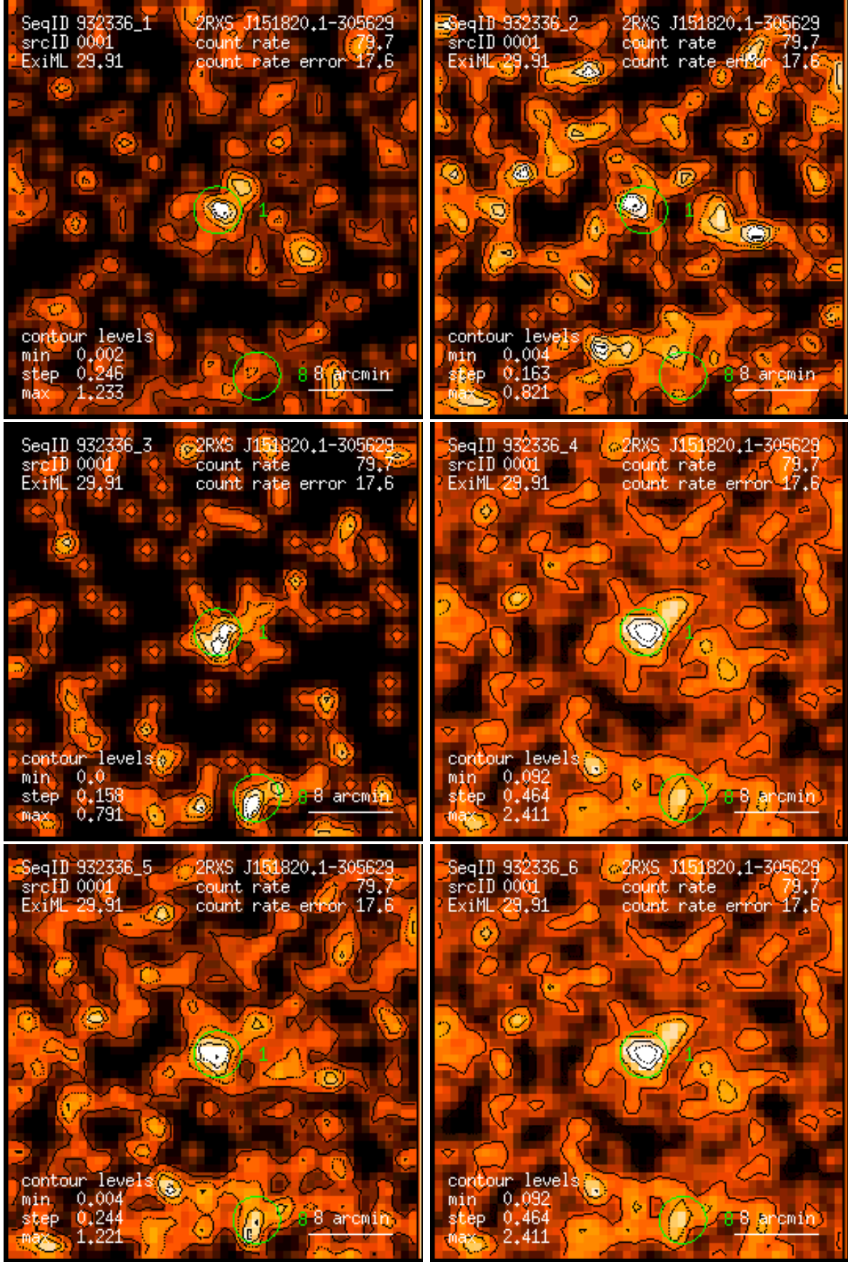
Figure 1: RASS 932336: detection 0001: band rate images, Gaussian filter: (1) PSPC channels 11 – 41, (2) 52 – 90, (3) 91 – 201, (4) 11 – 235, (5) 52 – 201, (6) 11 – 201. Broad band rates in counts/ks. Band rate contour levels in counts/ks/arcmin 2 .
