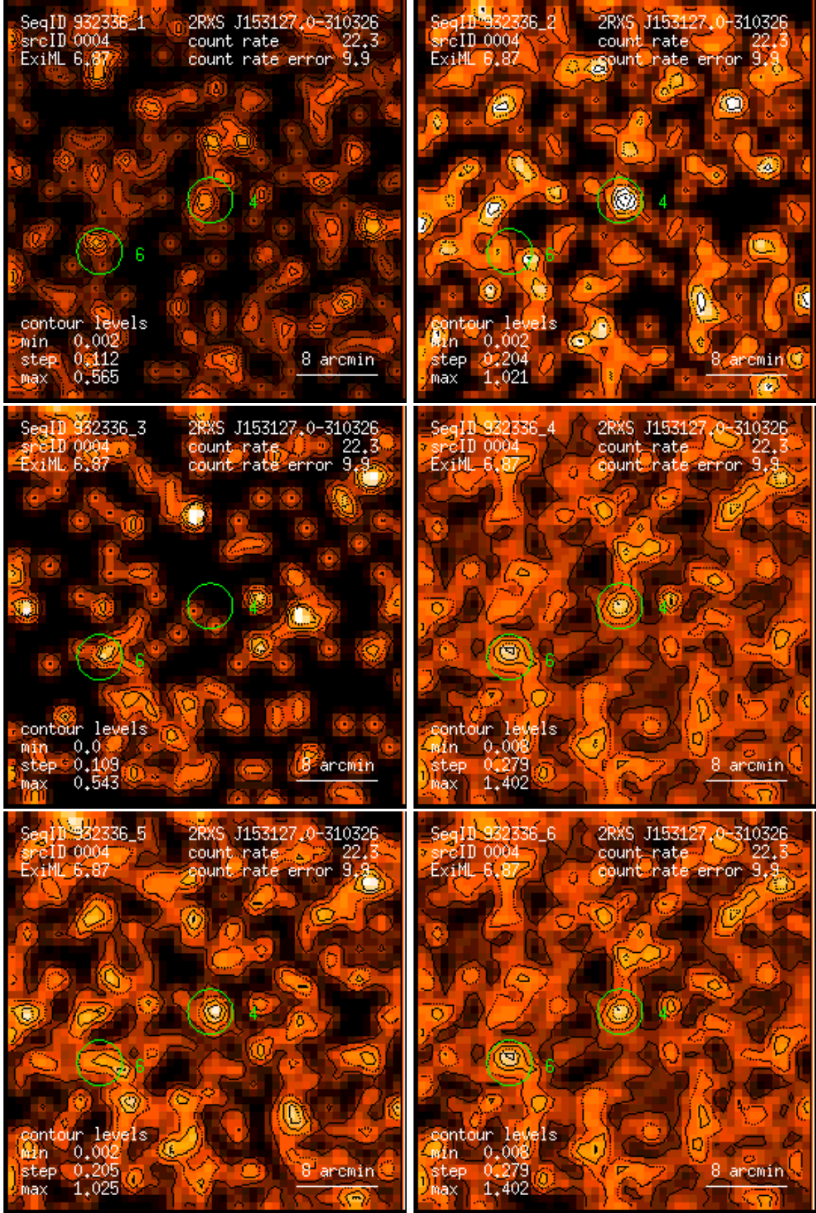
Figure 4: RASS 932336: detection 0004: band rate images, Gaussian filter: (1) PSPC channels 11 – 41, (2) 52 – 90, (3) 91 – 201, (4) 11 – 235, (5) 52 – 201, (6) 11 – 201. Broad band rates in counts/ks. Band rate contour levels in counts/ks/arcmin 2 .
