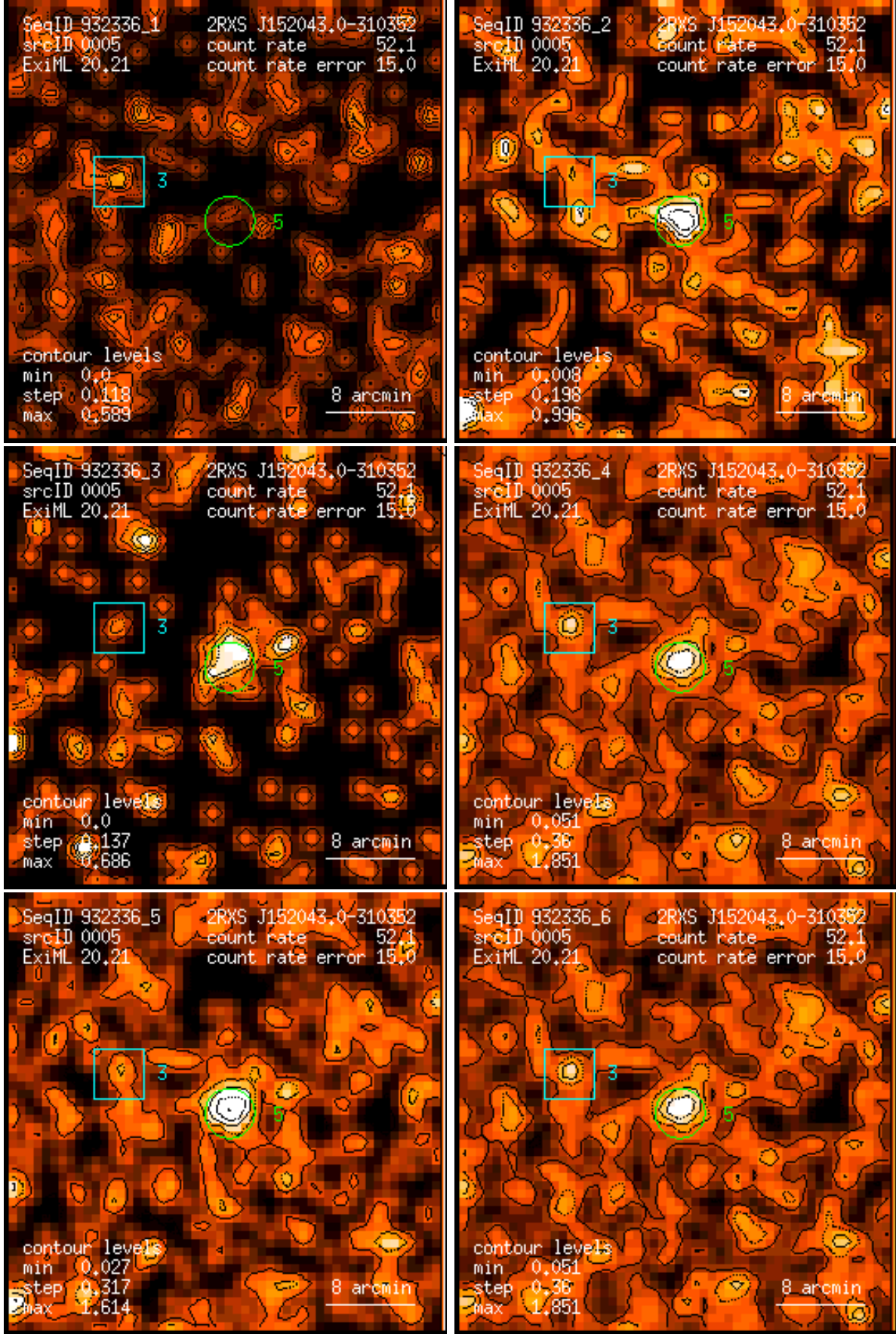
Figure 5: RASS 932336: detection 0005: band rate images, Gaussian filter: (1) PSPC channels 11 – 41, (2) 52 – 90, (3) 91 – 201, (4) 11 – 235, (5) 52 – 201, (6) 11 – 201. Broad band rates in counts/ks. Band rate contour levels in counts/ks/arcmin 2 .
