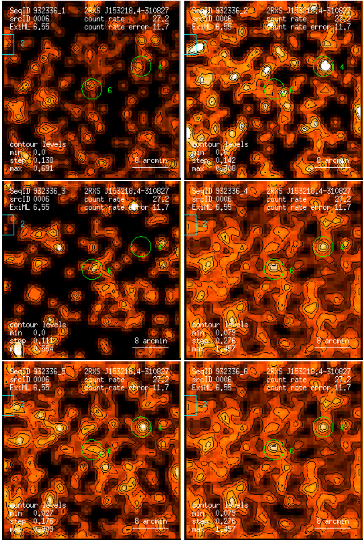
Figure 6: RASS 932336: detection 0006: band rate images, Gaussian filter: (1) PSPC channels 11 – 41, (2) 52 – 90, (3) 91 – 201, (4) 11 – 235, (5) 52 – 201, (6) 11 – 201. Broad band rates in counts/ks. Band rate contour levels in counts/ks/arcmin 2 .
