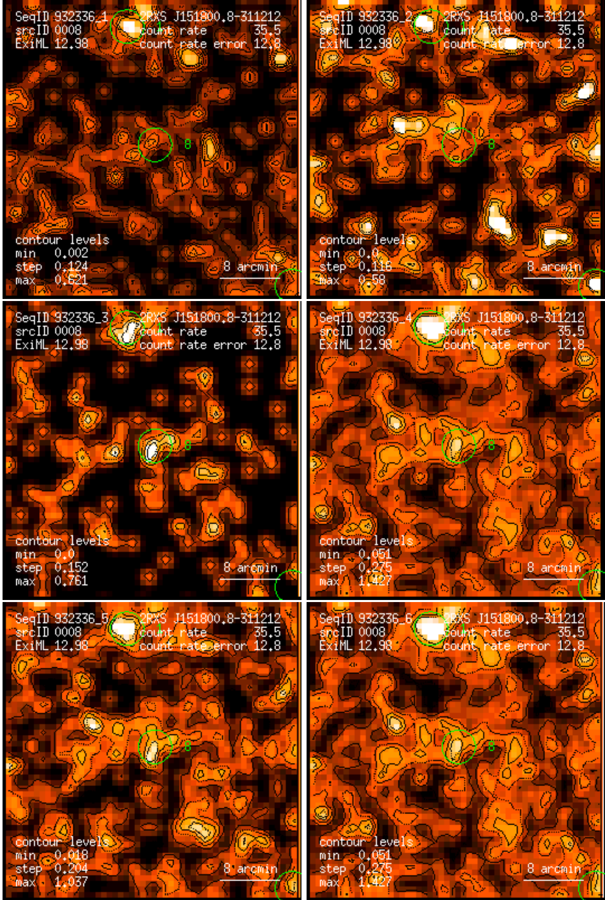
Figure 8: RASS 932336: detection 0008: band rate images, Gaussian filter: (1) PSPC channels 11 – 41, (2) 52 – 90, (3) 91 – 201, (4) 11 – 235, (5) 52 – 201, (6) 11 – 201. Broad band rates in counts/ks. Band rate contour levels in counts/ks/arcmin 2 .
