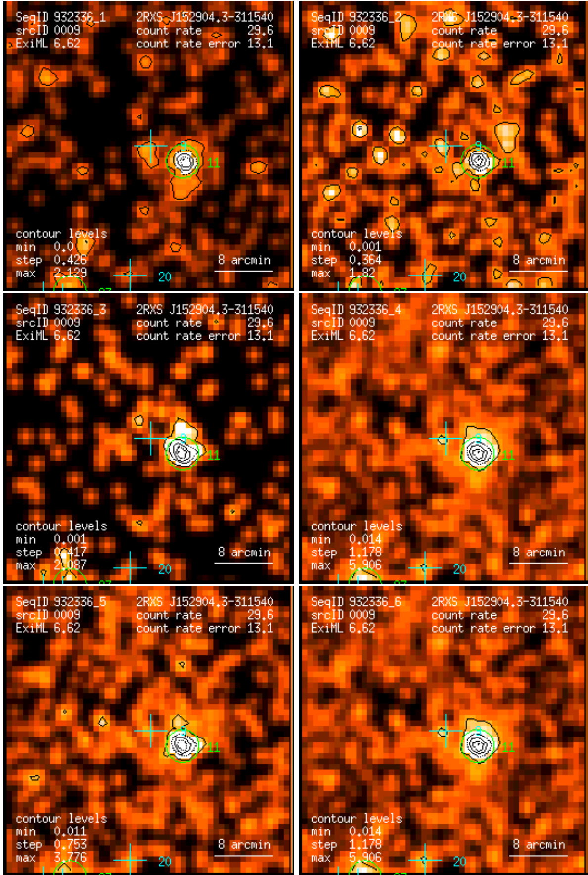
Figure 9: RASS 932336: detection 0009: band rate images, Gaussian filter: (1) PSPC channels 11 – 41, (2) 52 – 90, (3) 91 – 201, (4) 11 – 235, (5) 52 – 201, (6) 11 – 201. Broad band rates in counts/ks. Band rate contour levels in counts/ks/arcmin 2 .
