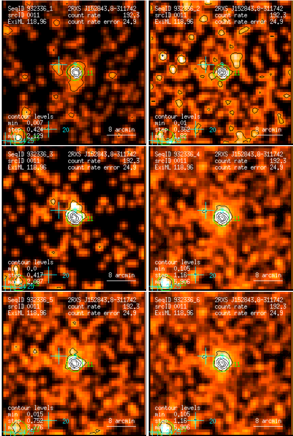
Figure 11: RASS 932336: detection 0011: band rate images, Gaussian filter: (1) PSPC channels 11 – 41, (2) 52 – 90, (3) 91 – 201, (4) 11 – 235, (5) 52 – 201, (6) 11 – 201. Broad band rates in counts/ks. Band rate contour levels in counts/ks/arcmin 2 .
