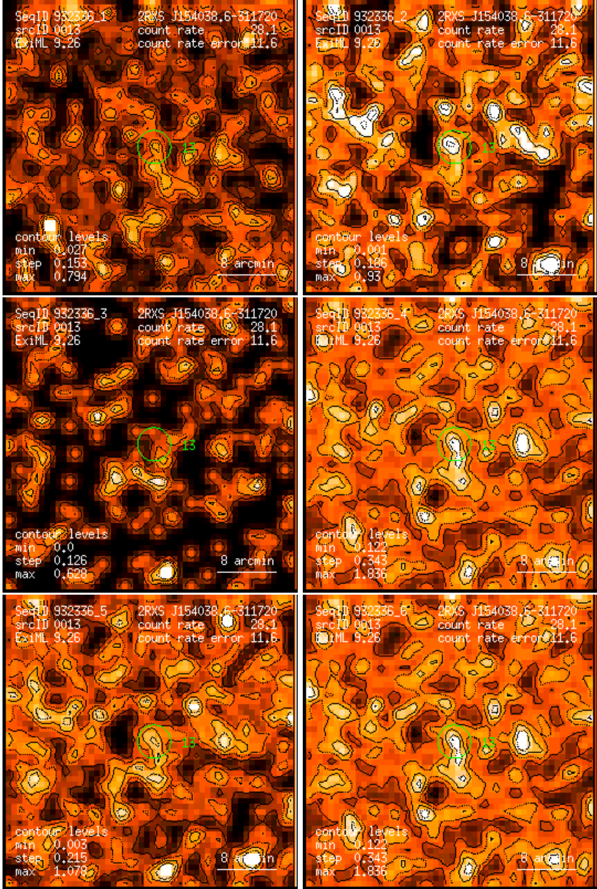
Figure 13: RASS 932336: detection 0013: band rate images, Gaussian filter: (1) PSPC channels 11 – 41, (2) 52 – 90, (3) 91 – 201, (4) 11 – 235, (5) 52 – 201, (6) 11 – 201. Broad band rates in counts/ks. Band rate contour levels in counts/ks/arcmin 2 .
