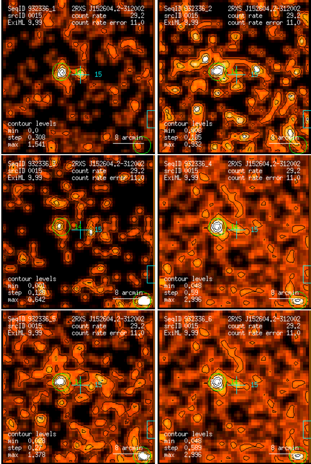
Figure 15: RASS 932336: detection 0015: band rate images, Gaussian filter: (1) PSPC channels 11 – 41, (2) 52 – 90, (3) 91 – 201, (4) 11 – 235, (5) 52 – 201, (6) 11 – 201. Broad band rates in counts/ks. Band rate contour levels in counts/ks/arcmin 2 .
