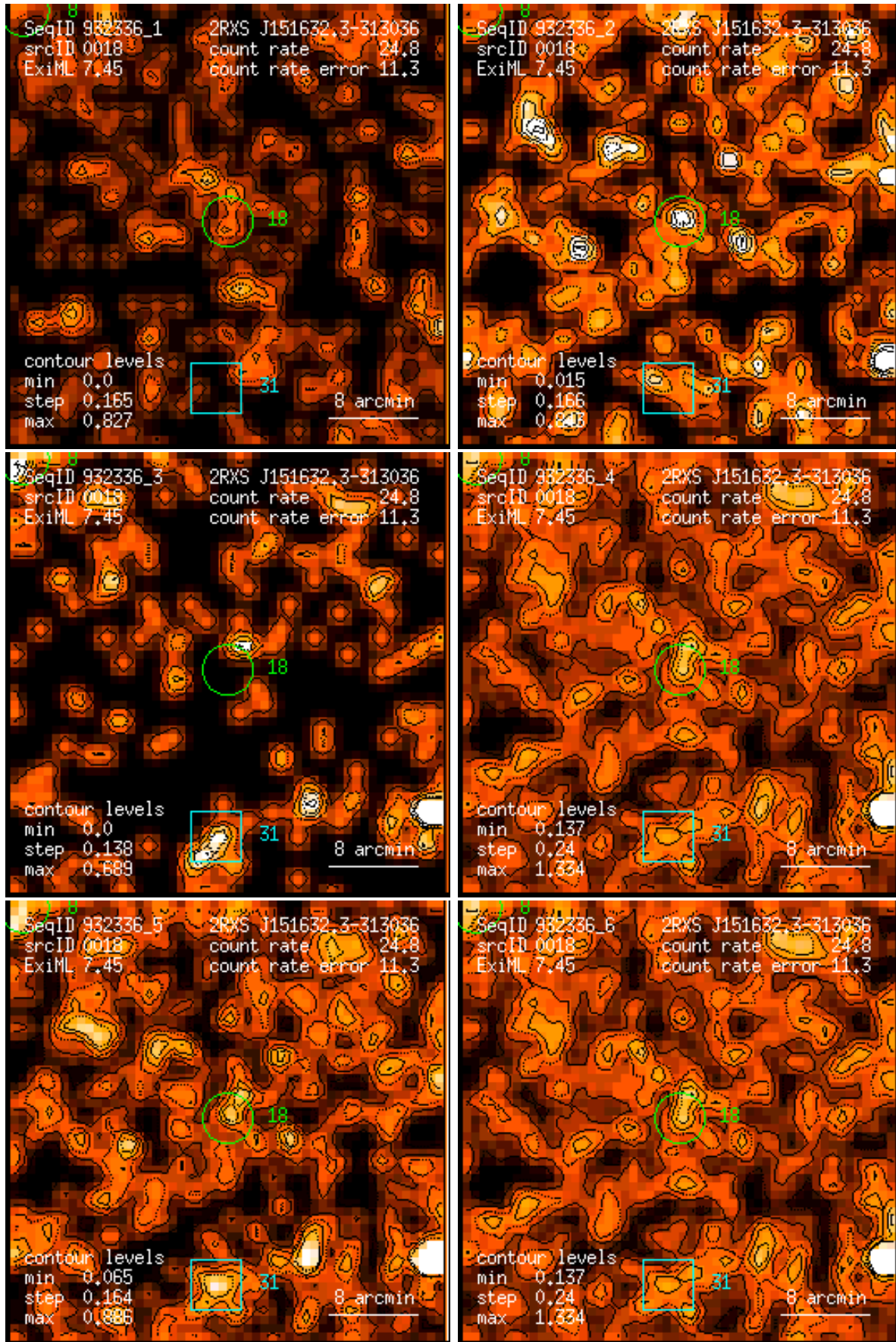
Figure 18: RASS 932336: detection 0018: band rate images, Gaussian filter: (1) PSPC channels 11 – 41, (2) 52 – 90, (3) 91 – 201, (4) 11 – 235, (5) 52 – 201, (6) 11 – 201. Broad band rates in counts/ks. Band rate contour levels in counts/ks/arcmin 2 .
