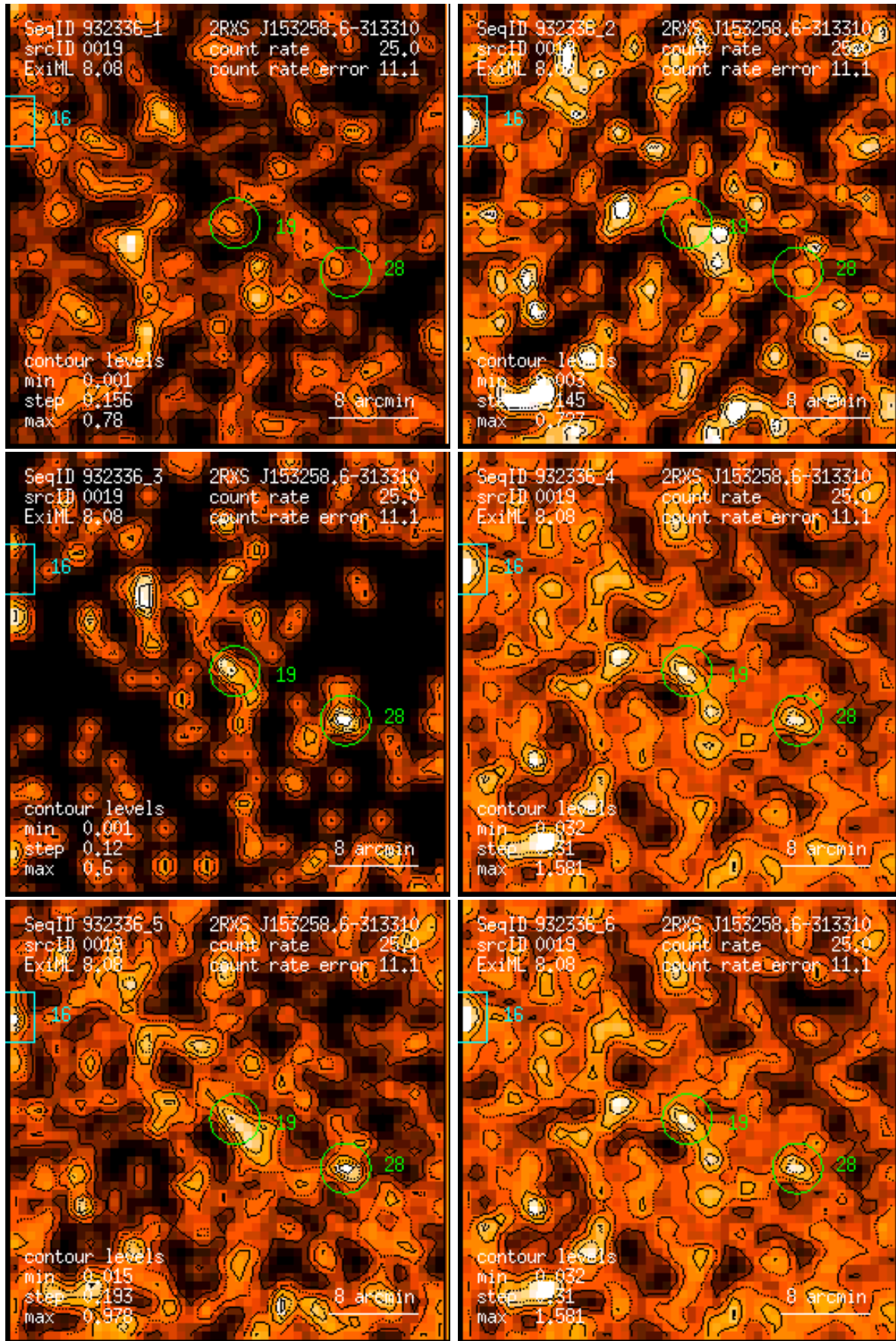
Figure 19: RASS 932336: detection 0019: band rate images, Gaussian filter: (1) PSPC channels 11 – 41, (2) 52 – 90, (3) 91 – 201, (4) 11 – 235, (5) 52 – 201, (6) 11 – 201. Broad band rates in counts/ks. Band rate contour levels in counts/ks/arcmin 2 .
