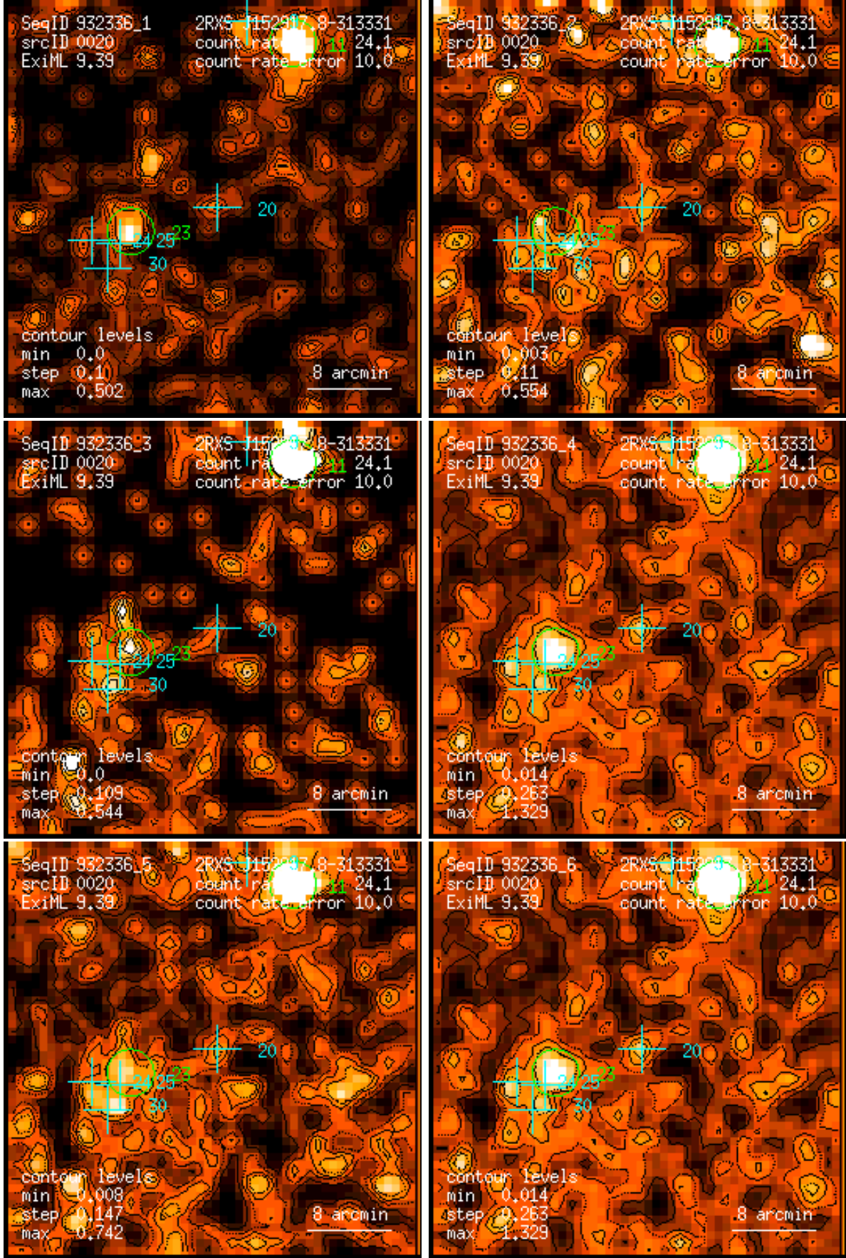
Figure 20: RASS 932336: detection 0020: band rate images, Gaussian filter: (1) PSPC channels 11 – 41, (2) 52 – 90, (3) 91 – 201, (4) 11 – 235, (5) 52 – 201, (6) 11 – 201. Broad band rates in counts/ks. Band rate contour levels in counts/ks/arcmin 2 .
