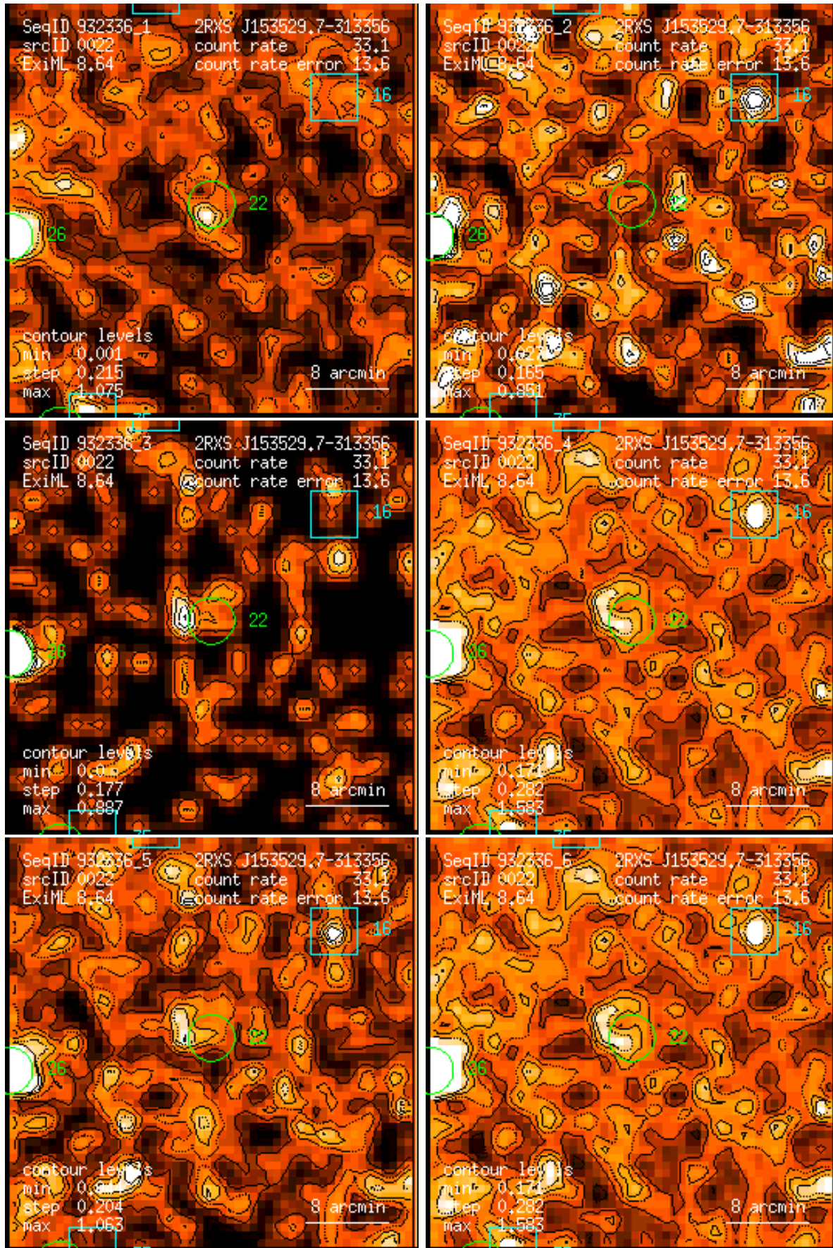
Figure 22: RASS 932336: detection 0022: band rate images, Gaussian filter: (1) PSPC channels 11 – 41, (2) 52 – 90, (3) 91 – 201, (4) 11 – 235, (5) 52 – 201, (6) 11 – 201. Broad band rates in counts/ks. Band rate contour levels in counts/ks/arcmin 2 .
