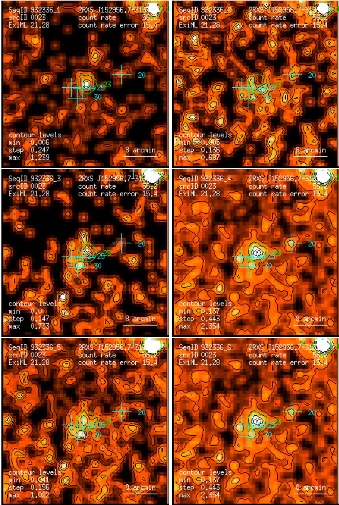
Figure 23: RASS 932336: detection 0023: band rate images, Gaussian filter: (1) PSPC channels 11 – 41, (2) 52 – 90, (3) 91 – 201, (4) 11 – 235, (5) 52 – 201, (6) 11 – 201. Broad band rates in counts/ks. Band rate contour levels in counts/ks/arcmin 2 .
