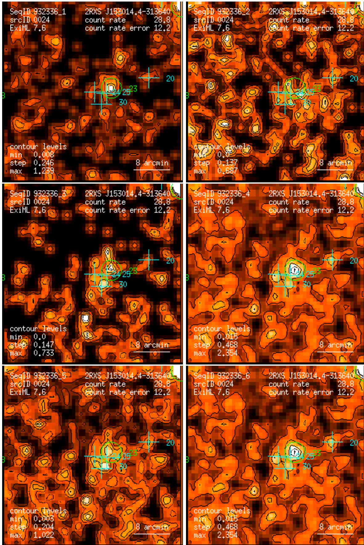
Figure 24: RASS 932336: detection 0024: band rate images, Gaussian filter: (1) PSPC channels 11 – 41, (2) 52 – 90, (3) 91 – 201, (4) 11 – 235, (5) 52 – 201, (6) 11 – 201. Broad band rates in counts/ks. Band rate contour levels in counts/ks/arcmin 2 .
