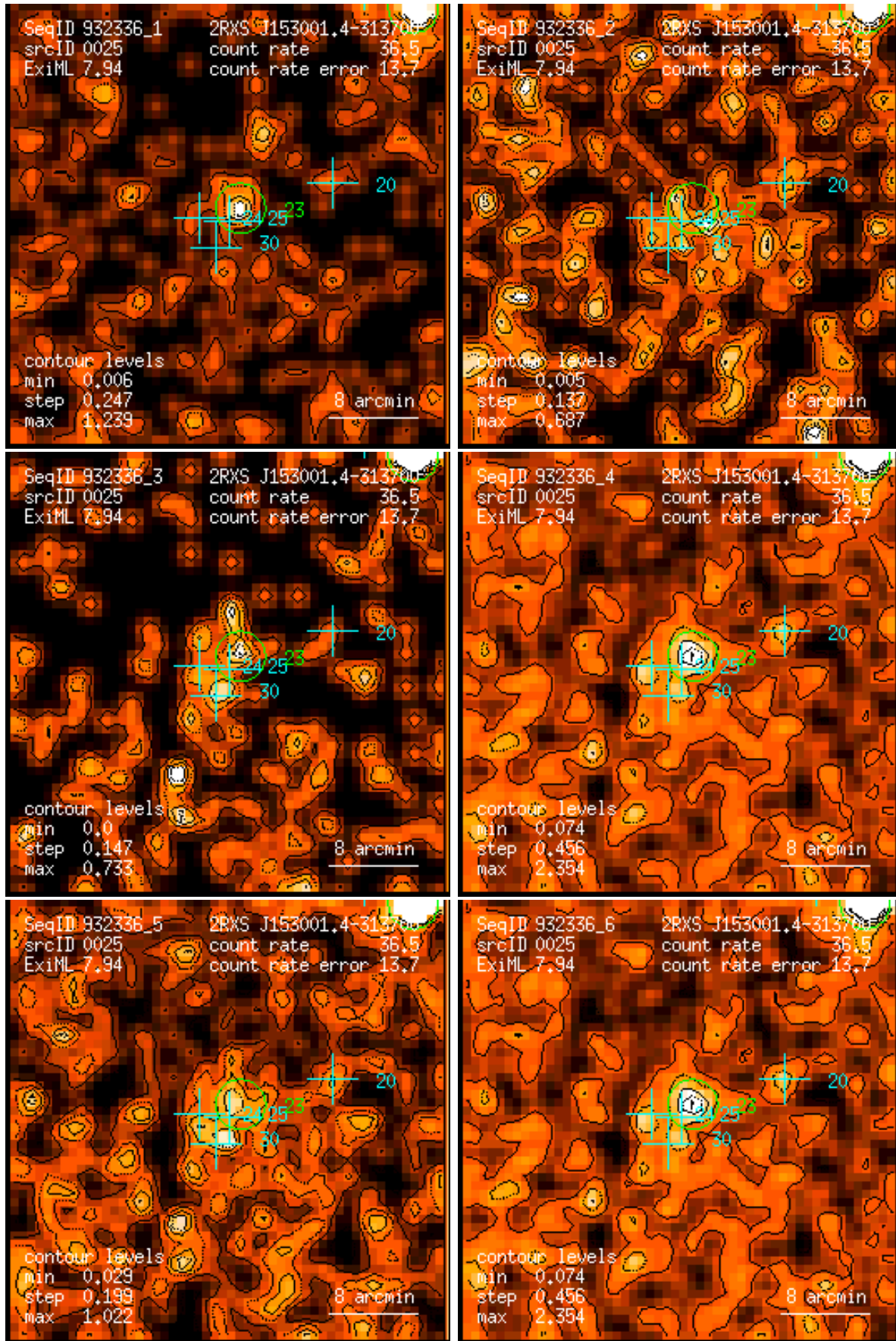
Figure 25: RASS 932336: detection 0025: band rate images, Gaussian filter: (1) PSPC channels 11 – 41, (2) 52 – 90, (3) 91 – 201, (4) 11 – 235, (5) 52 – 201, (6) 11 – 201. Broad band rates in counts/ks. Band rate contour levels in counts/ks/arcmin 2 .
