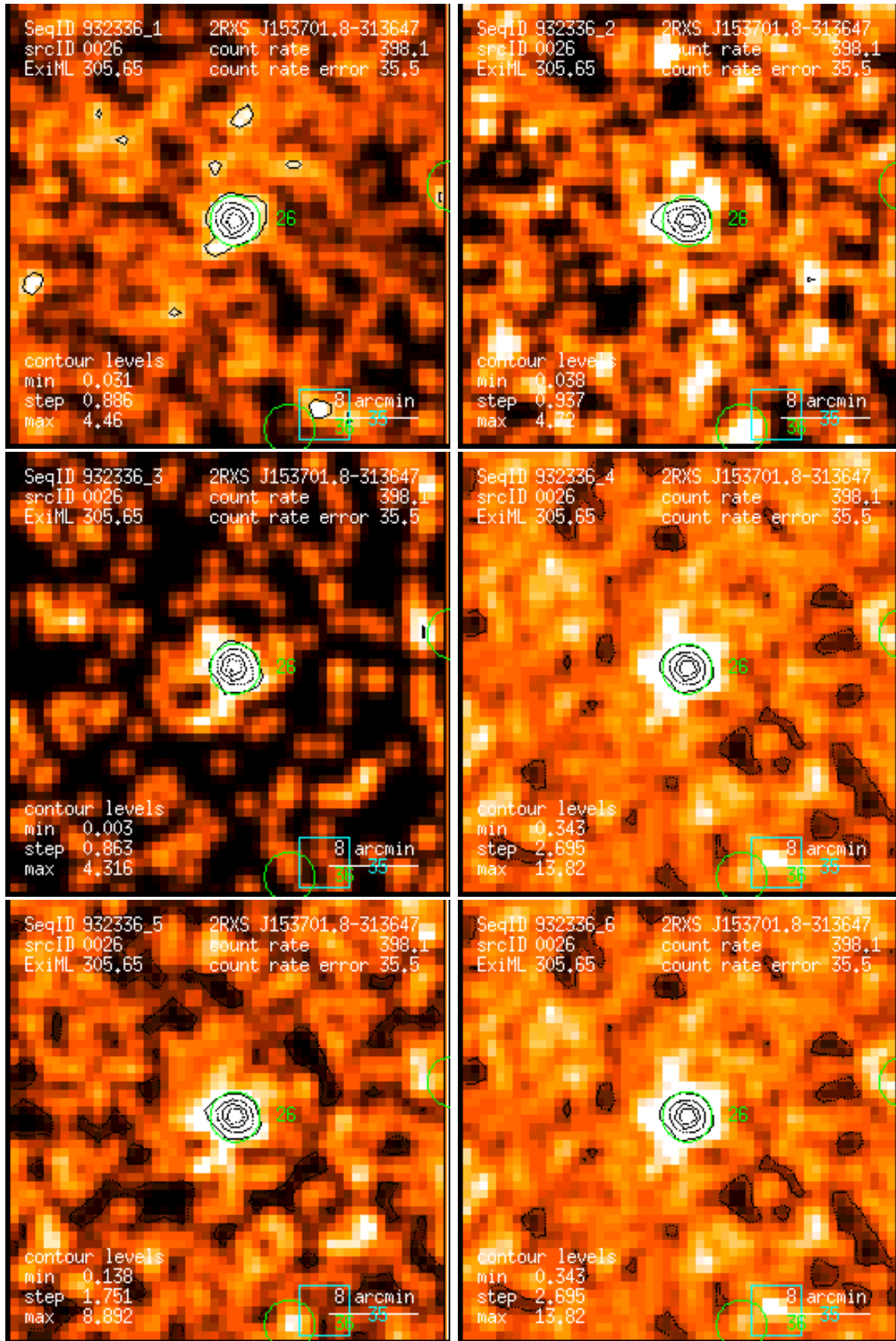
Figure 26: RASS 932336: detection 0026: band rate images, Gaussian filter: (1) PSPC channels 11 – 41, (2) 52 – 90, (3) 91 – 201, (4) 11 – 235, (5) 52 – 201, (6) 11 – 201. Broad band rates in counts/ks. Band rate contour levels in counts/ks/arcmin 2 .
