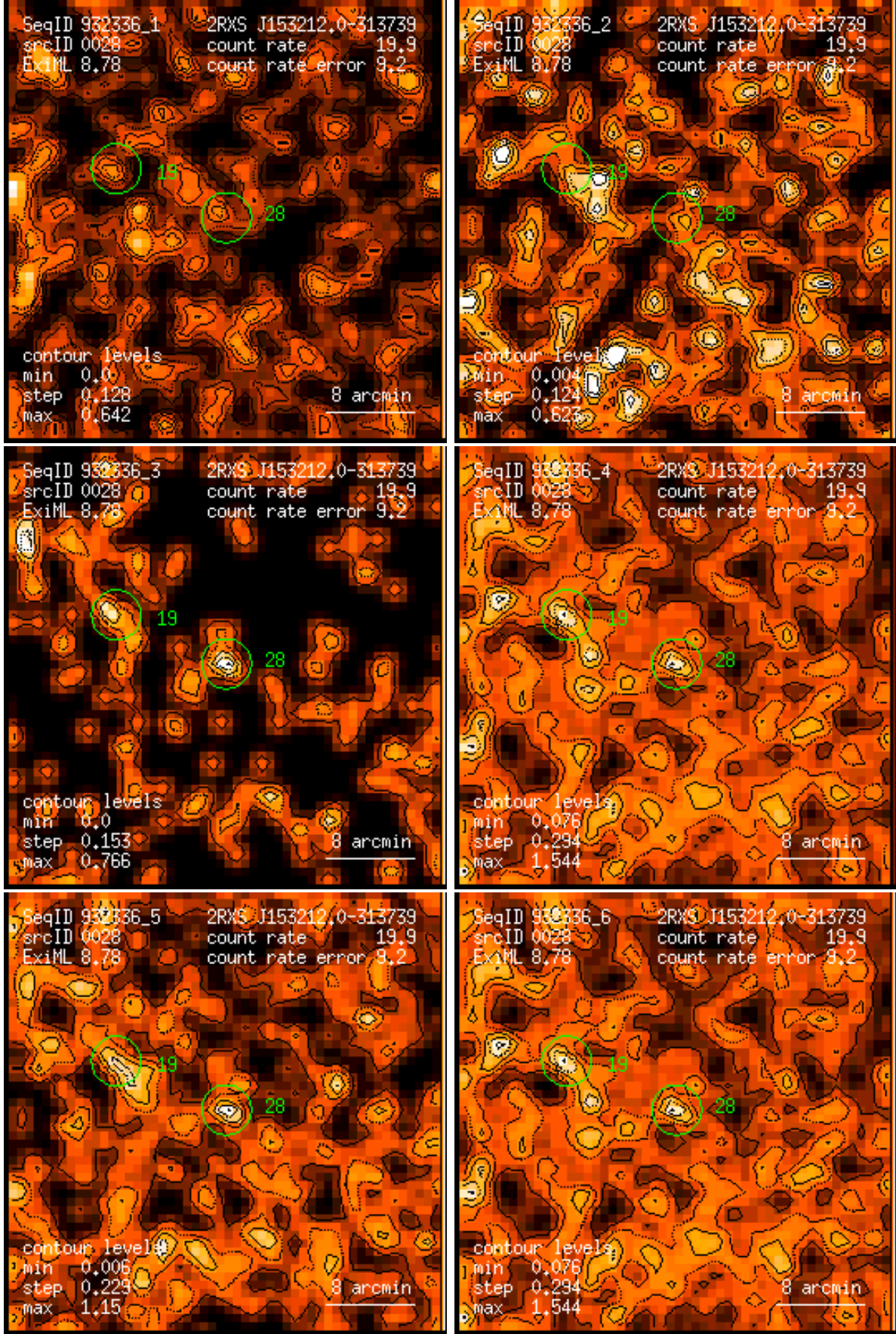
Figure 28: RASS 932336: detection 0028: band rate images, Gaussian filter: (1) PSPC channels 11 – 41, (2) 52 – 90, (3) 91 – 201, (4) 11 – 235, (5) 52 – 201, (6) 11 – 201. Broad band rates in counts/ks. Band rate contour levels in counts/ks/arcmin 2 .
