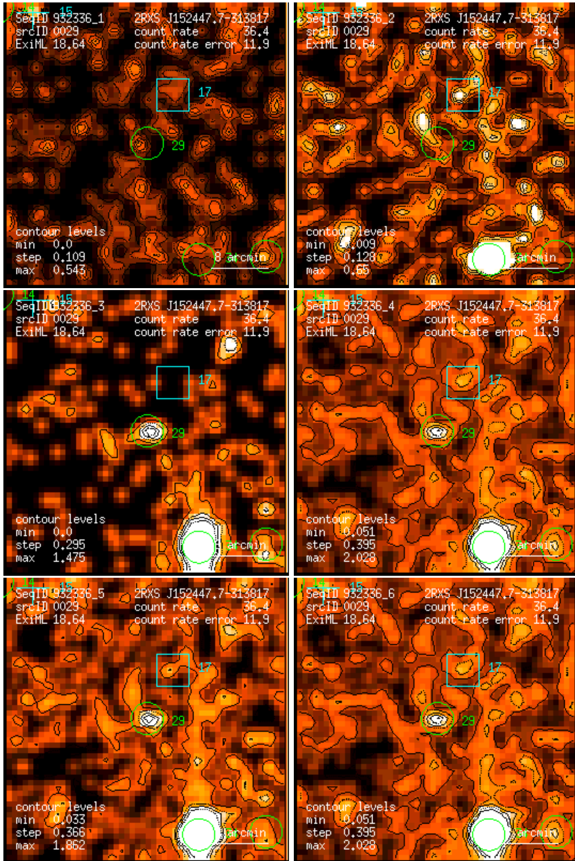
Figure 29: RASS 932336: detection 0029: band rate images, Gaussian filter: (1) PSPC channels 11 – 41, (2) 52 – 90, (3) 91 – 201, (4) 11 – 235, (5) 52 – 201, (6) 11 – 201. Broad band rates in counts/ks. Band rate contour levels in counts/ks/arcmin 2 .
