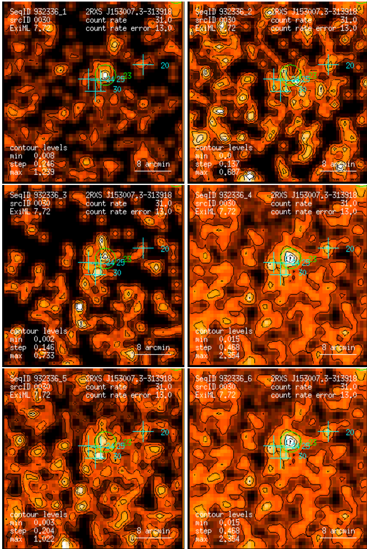
Figure 30: RASS 932336: detection 0030: band rate images, Gaussian filter: (1) PSPC channels 11 – 41, (2) 52 – 90, (3) 91 – 201, (4) 11 – 235, (5) 52 – 201, (6) 11 – 201. Broad band rates in counts/ks. Band rate contour levels in counts/ks/arcmin 2 .
