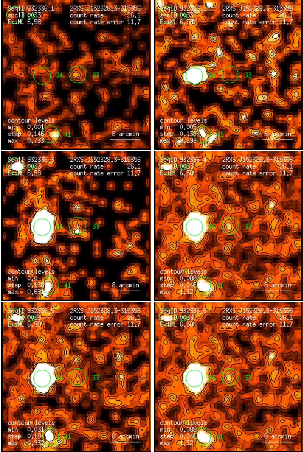
Figure 33: RASS 932336: detection 0033: band rate images, Gaussian filter: (1) PSPC channels 11 – 41, (2) 52 – 90, (3) 91 – 201, (4) 11 – 235, (5) 52 – 201, (6) 11 – 201. Broad band rates in counts/ks. Band rate contour levels in counts/ks/arcmin 2 .
