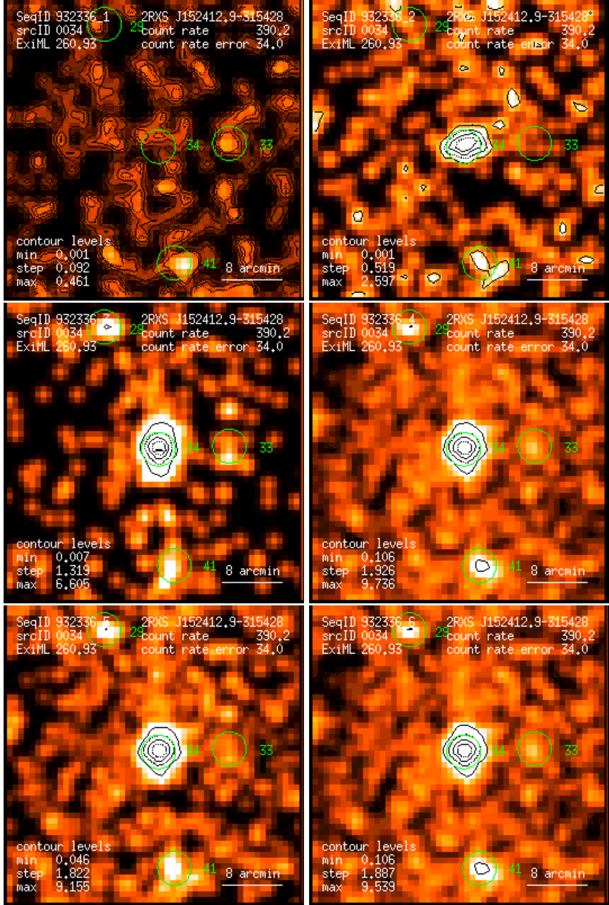
Figure 34: RASS 932336: detection 0034: band rate images, Gaussian filter: (1) PSPC channels 11 – 41, (2) 52 – 90, (3) 91 – 201, (4) 11 – 235, (5) 52 – 201, (6) 11 – 201. Broad band rates in counts/ks. Band rate contour levels in counts/ks/arcmin 2 .
