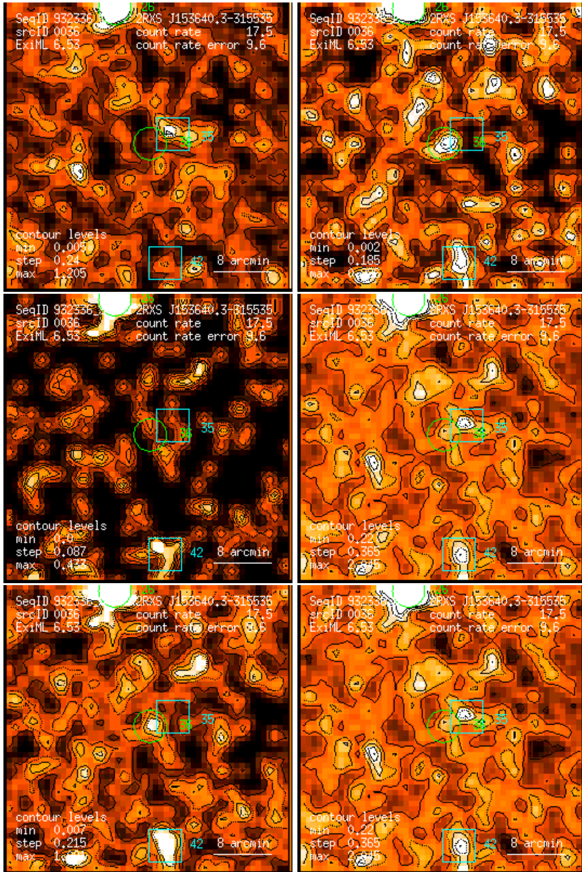
Figure 36: RASS 932336: detection 0036: band rate images, Gaussian filter: (1) PSPC channels 11 – 41, (2) 52 – 90, (3) 91 – 201, (4) 11 – 235, (5) 52 – 201, (6) 11 – 201. Broad band rates in counts/ks. Band rate contour levels in counts/ks/arcmin 2 .
