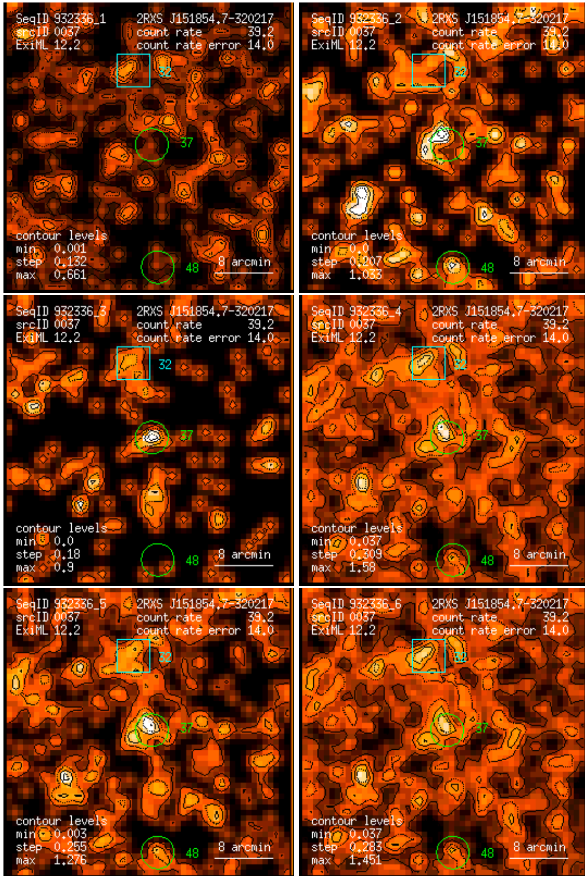
Figure 37: RASS 932336: detection 0037: band rate images, Gaussian filter: (1) PSPC channels 11 – 41, (2) 52 – 90, (3) 91 – 201, (4) 11 – 235, (5) 52 – 201, (6) 11 – 201. Broad band rates in counts/ks. Band rate contour levels in counts/ks/arcmin 2 .
