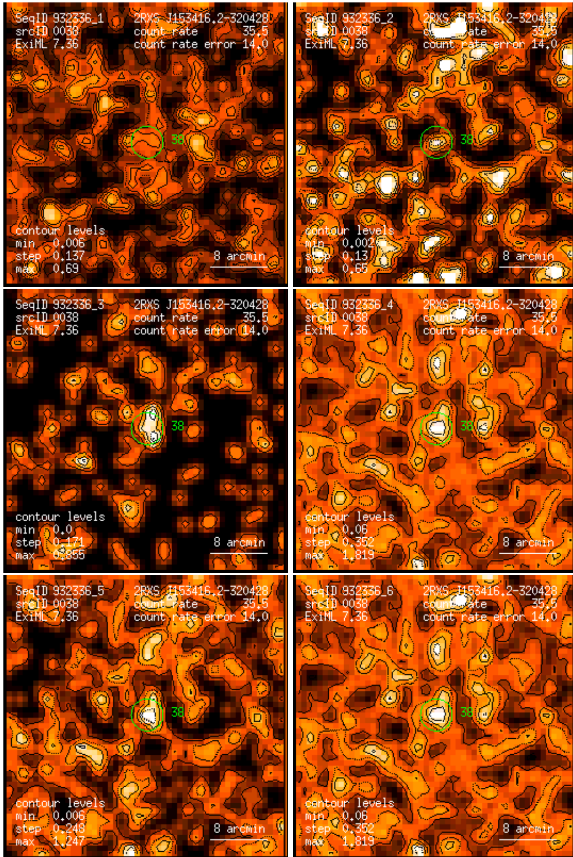
Figure 38: RASS 932336: detection 0038: band rate images, Gaussian filter: (1) PSPC channels 11 – 41, (2) 52 – 90, (3) 91 – 201, (4) 11 – 235, (5) 52 – 201, (6) 11 – 201. Broad band rates in counts/ks. Band rate contour levels in counts/ks/arcmin 2 .
