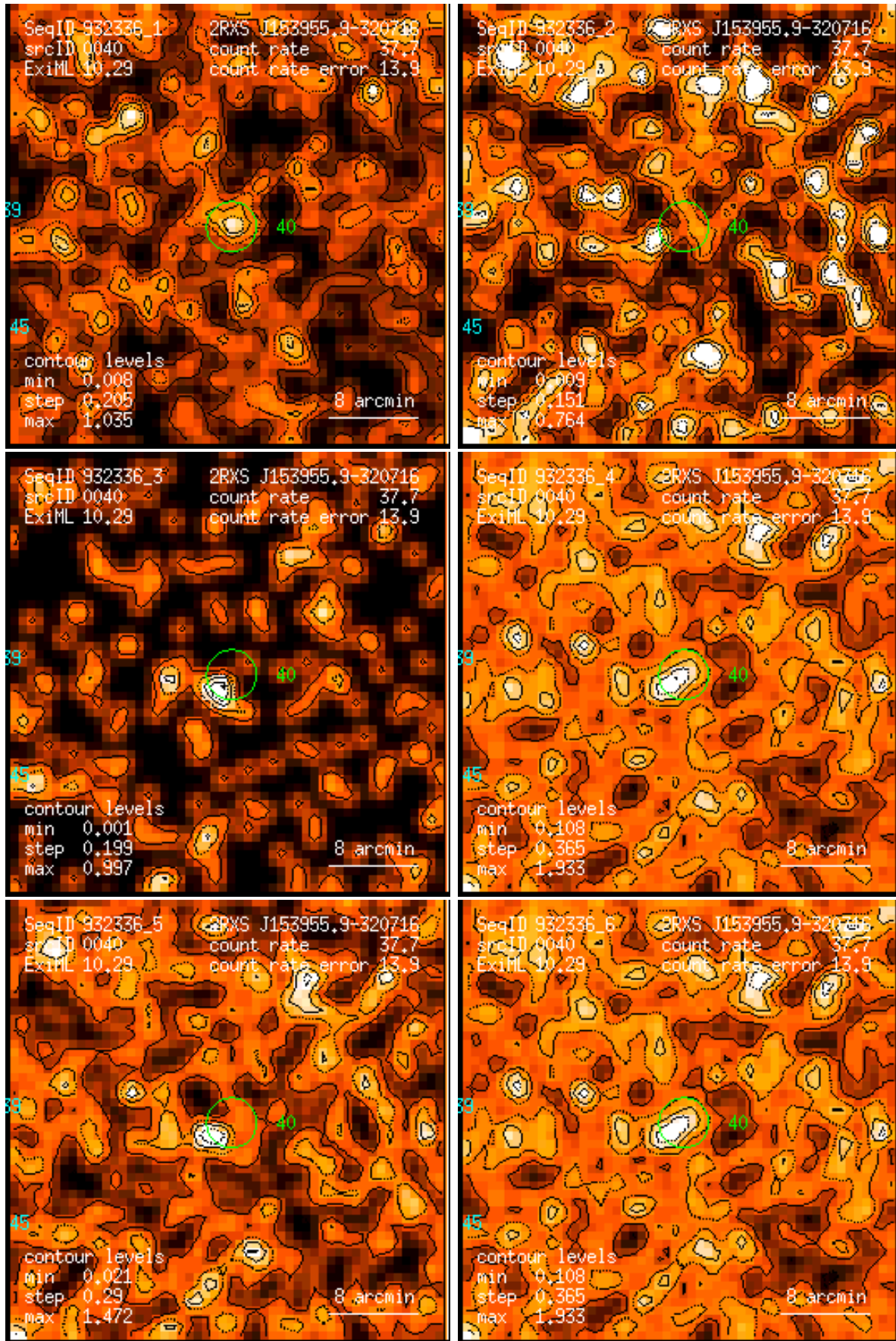
Figure 40: RASS 932336: detection 0040: band rate images, Gaussian filter: (1) PSPC channels 11 – 41, (2) 52 – 90, (3) 91 – 201, (4) 11 – 235, (5) 52 – 201, (6) 11 – 201. Broad band rates in counts/ks. Band rate contour levels in counts/ks/arcmin 2 .
