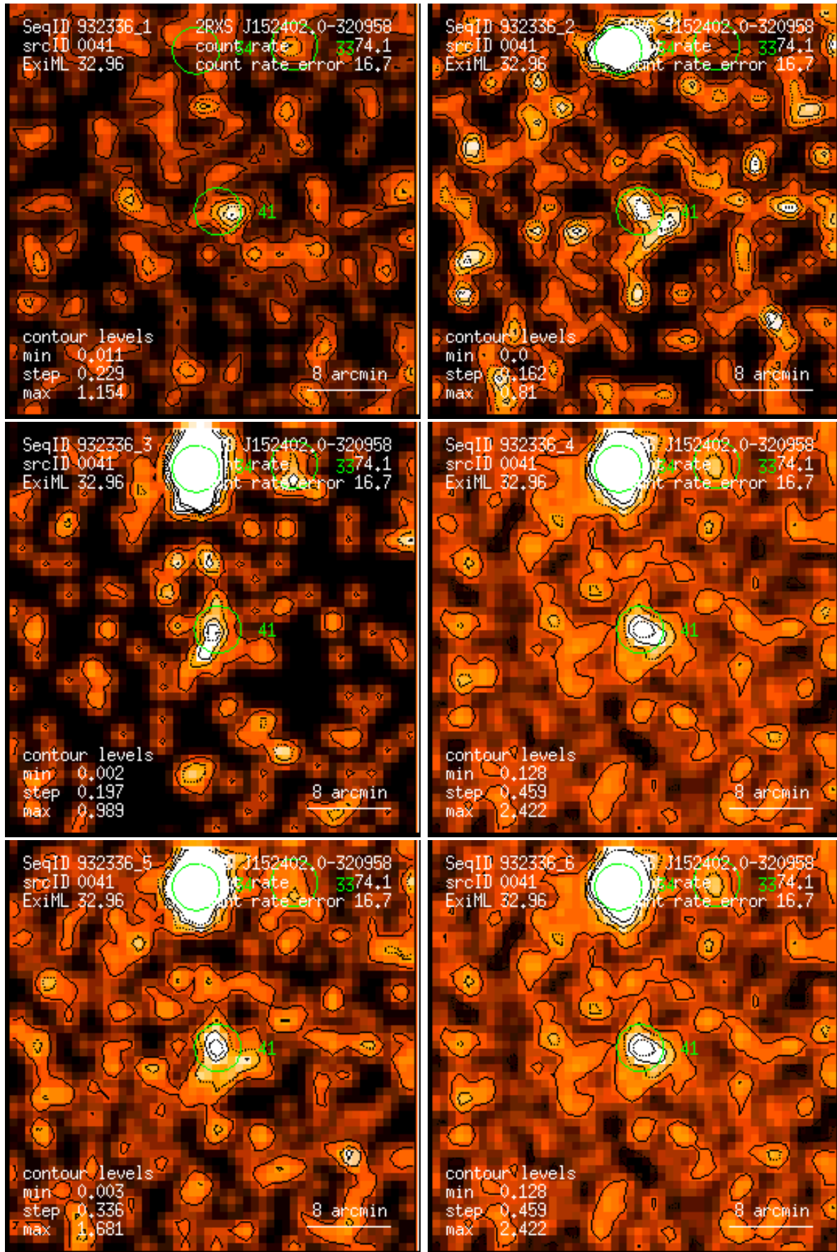
Figure 41: RASS 932336: detection 0041: band rate images, Gaussian filter: (1) PSPC channels 11 – 41, (2) 52 – 90, (3) 91 – 201, (4) 11 – 235, (5) 52 – 201, (6) 11 – 201. Broad band rates in counts/ks. Band rate contour levels in counts/ks/arcmin 2 .
