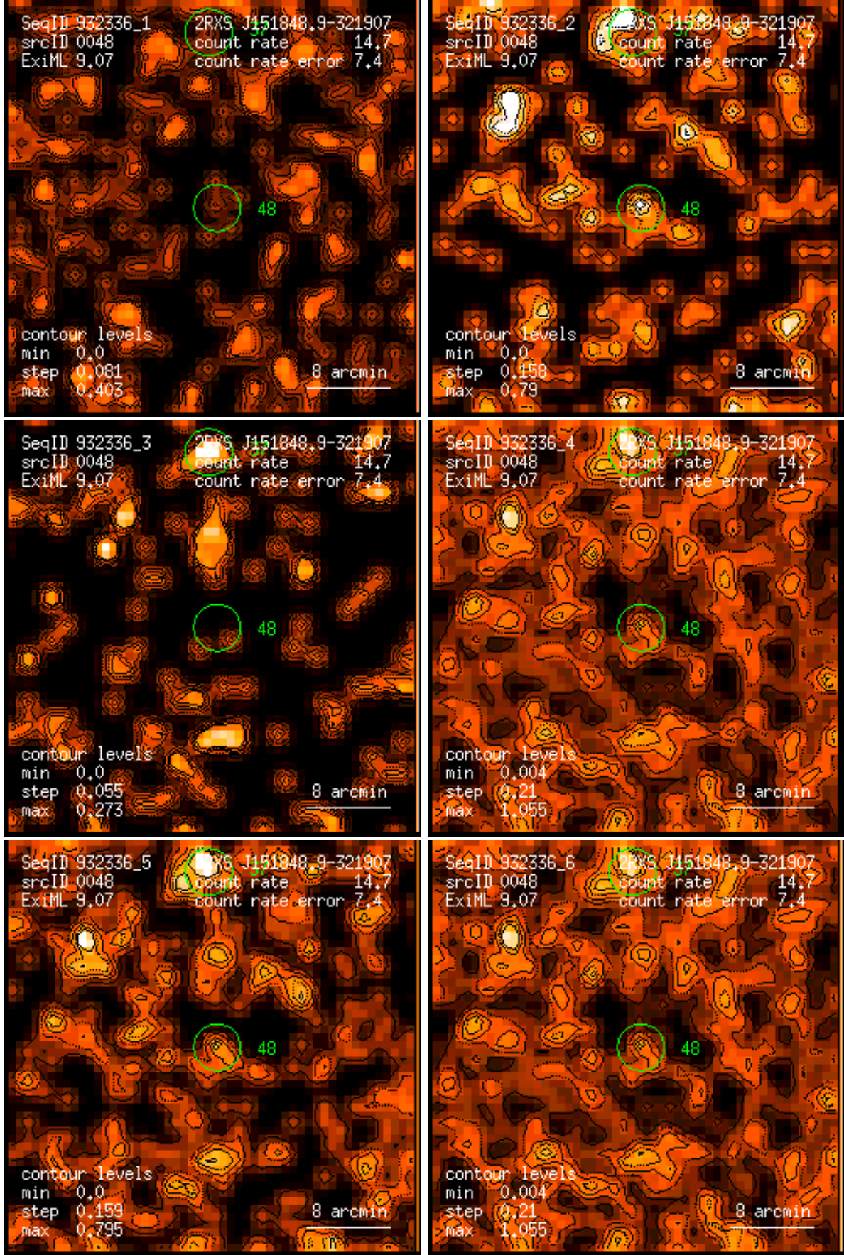
Figure 48: RASS 932336: detection 0048: band rate images, Gaussian filter: (1) PSPC channels 11 – 41, (2) 52 – 90, (3) 91 – 201, (4) 11 – 235, (5) 52 – 201, (6) 11 – 201. Broad band rates in counts/ks. Band rate contour levels in counts/ks/arcmin 2 .
