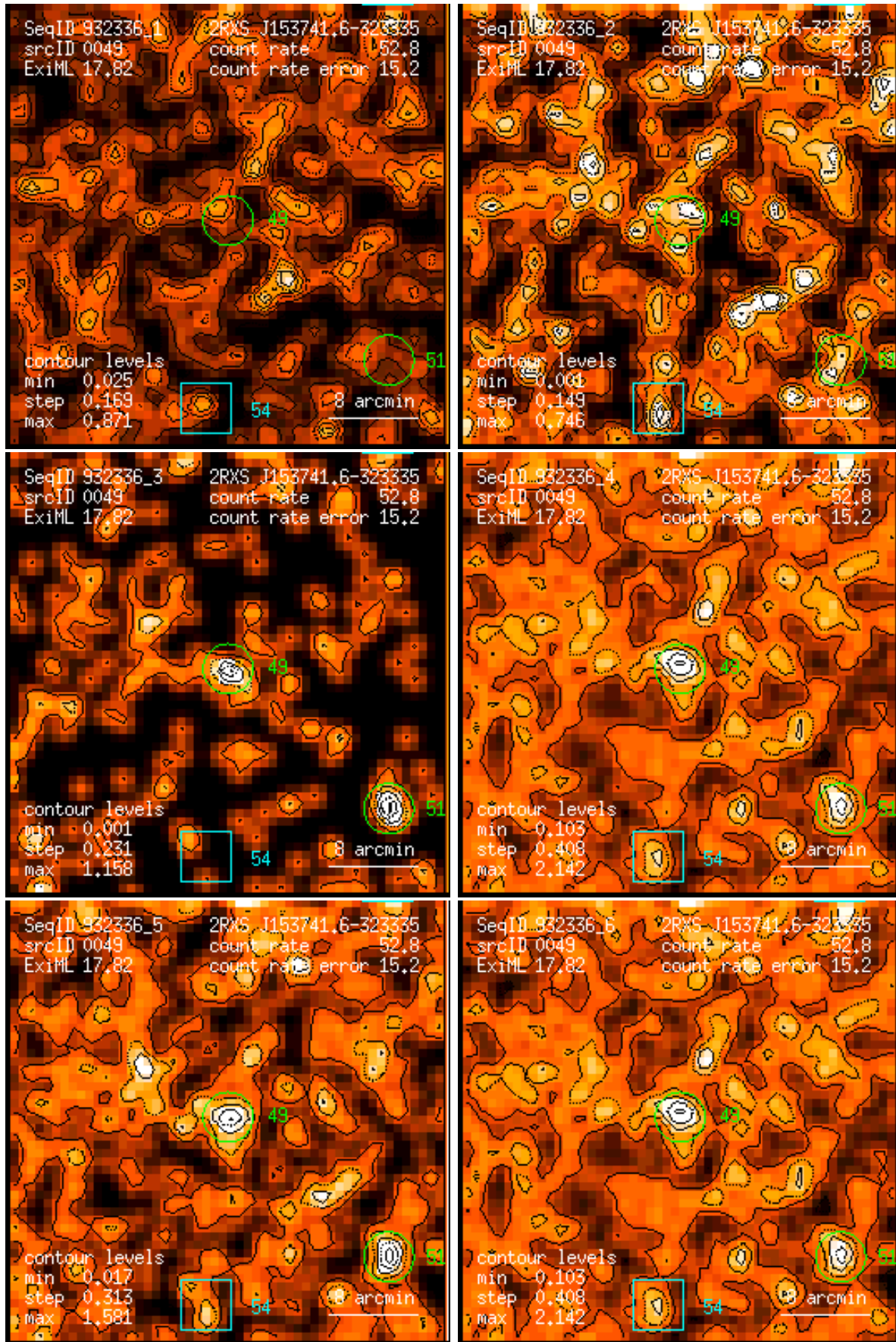
Figure 49: RASS 932336: detection 0049: band rate images, Gaussian filter: (1) PSPC channels 11 – 41, (2) 52 – 90, (3) 91 – 201, (4) 11 – 235, (5) 52 – 201, (6) 11 – 201. Broad band rates in counts/ks. Band rate contour levels in counts/ks/arcmin 2 .
