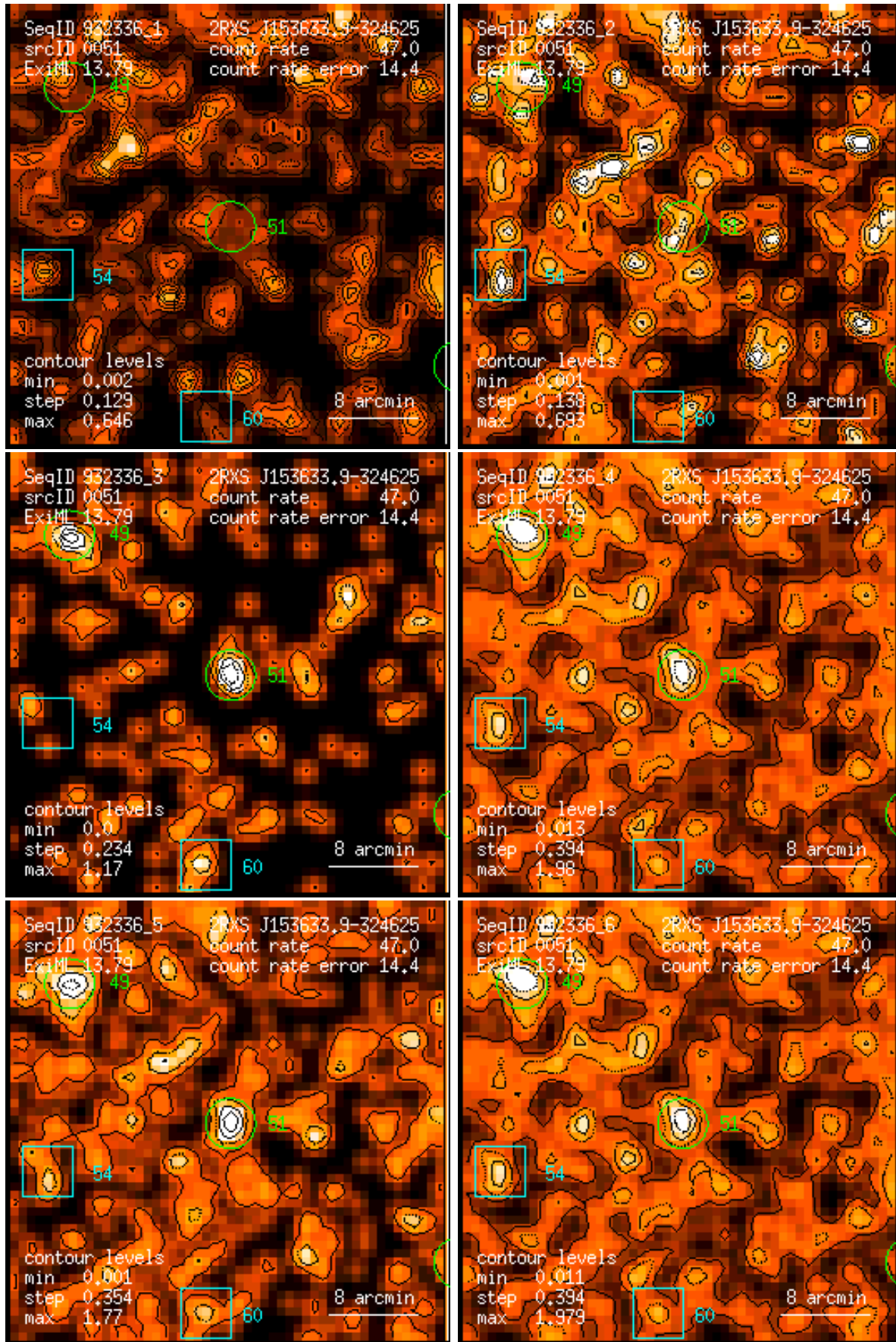
Figure 51: RASS 932336: detection 0051: band rate images, Gaussian filter: (1) PSPC channels 11 – 41, (2) 52 – 90, (3) 91 – 201, (4) 11 – 235, (5) 52 – 201, (6) 11 – 201. Broad band rates in counts/ks. Band rate contour levels in counts/ks/arcmin 2 .
