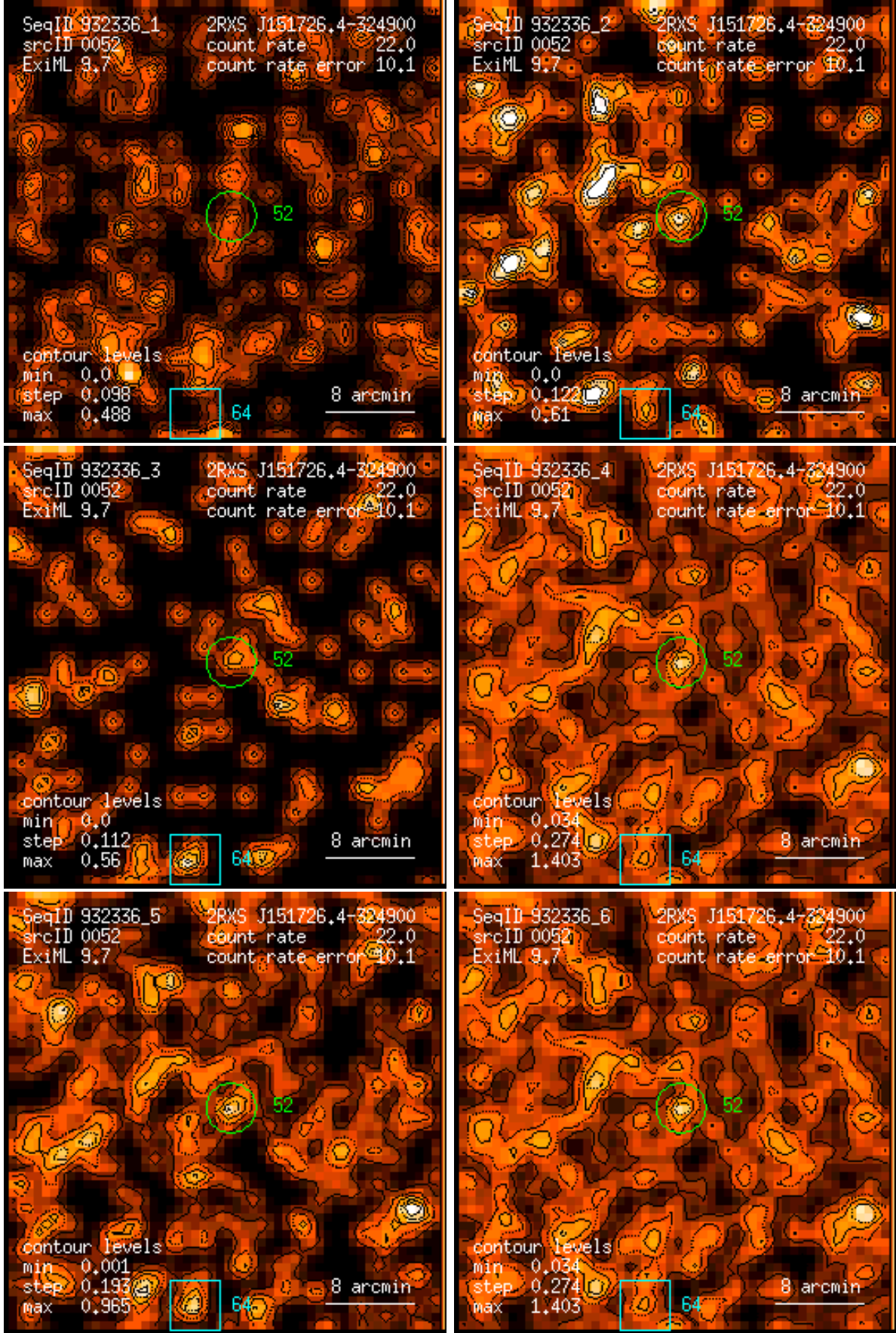
Figure 52: RASS 932336: detection 0052: band rate images, Gaussian filter: (1) PSPC channels 11 – 41, (2) 52 – 90, (3) 91 – 201, (4) 11 – 235, (5) 52 – 201, (6) 11 – 201. Broad band rates in counts/ks. Band rate contour levels in counts/ks/arcmin 2 .
