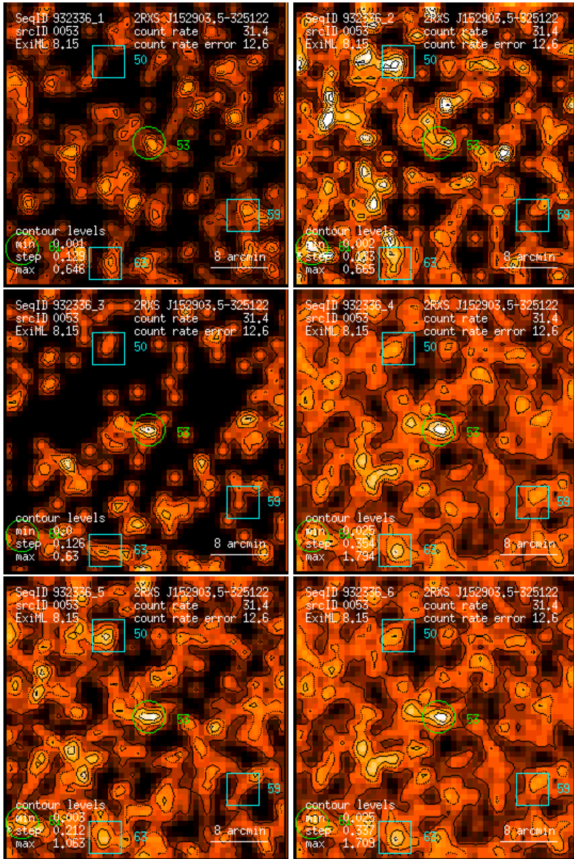
Figure 53: RASS 932336: detection 0053: band rate images, Gaussian filter: (1) PSPC channels 11 – 41, (2) 52 – 90, (3) 91 – 201, (4) 11 – 235, (5) 52 – 201, (6) 11 – 201. Broad band rates in counts/ks. Band rate contour levels in counts/ks/arcmin 2 .
