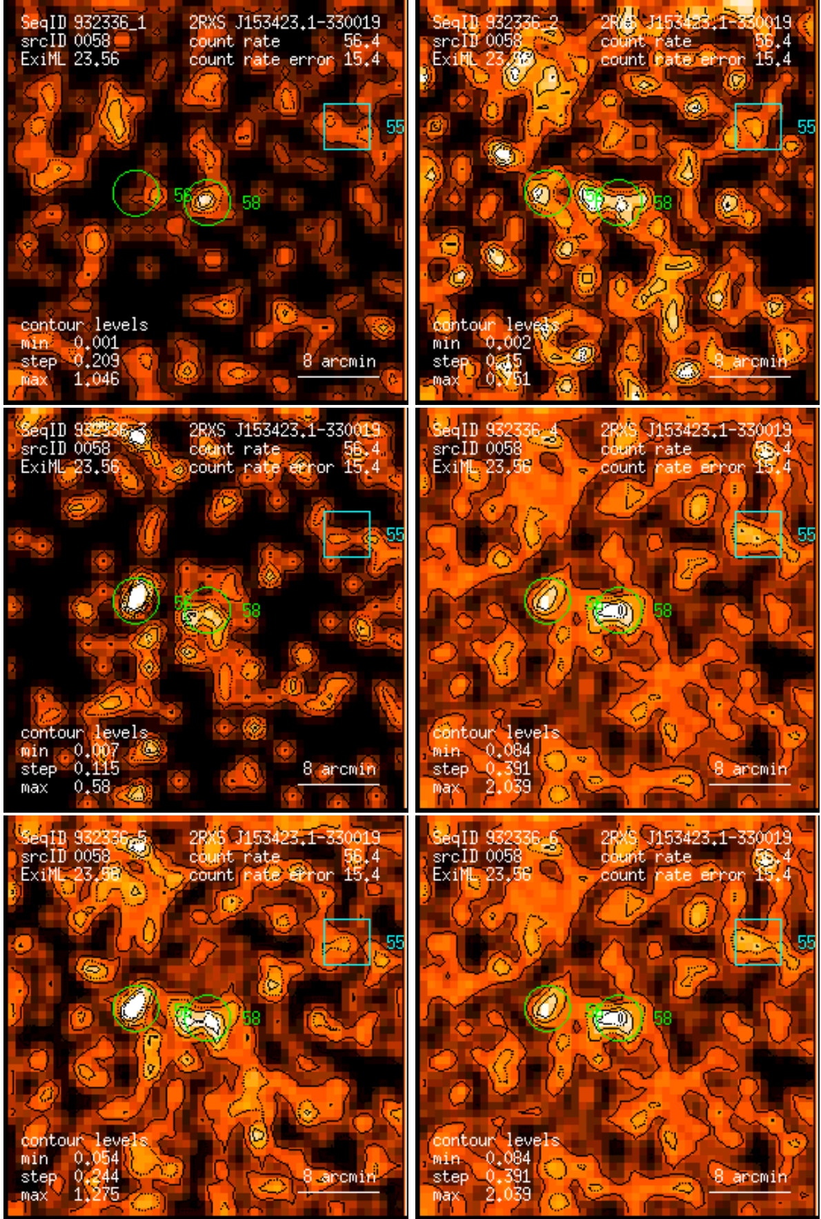
Figure 58: RASS 932336: detection 0058: band rate images, Gaussian filter: (1) PSPC channels 11 – 41, (2) 52 – 90, (3) 91 – 201, (4) 11 – 235, (5) 52 – 201, (6) 11 – 201. Broad band rates in counts/ks. Band rate contour levels in counts/ks/arcmin 2 .
