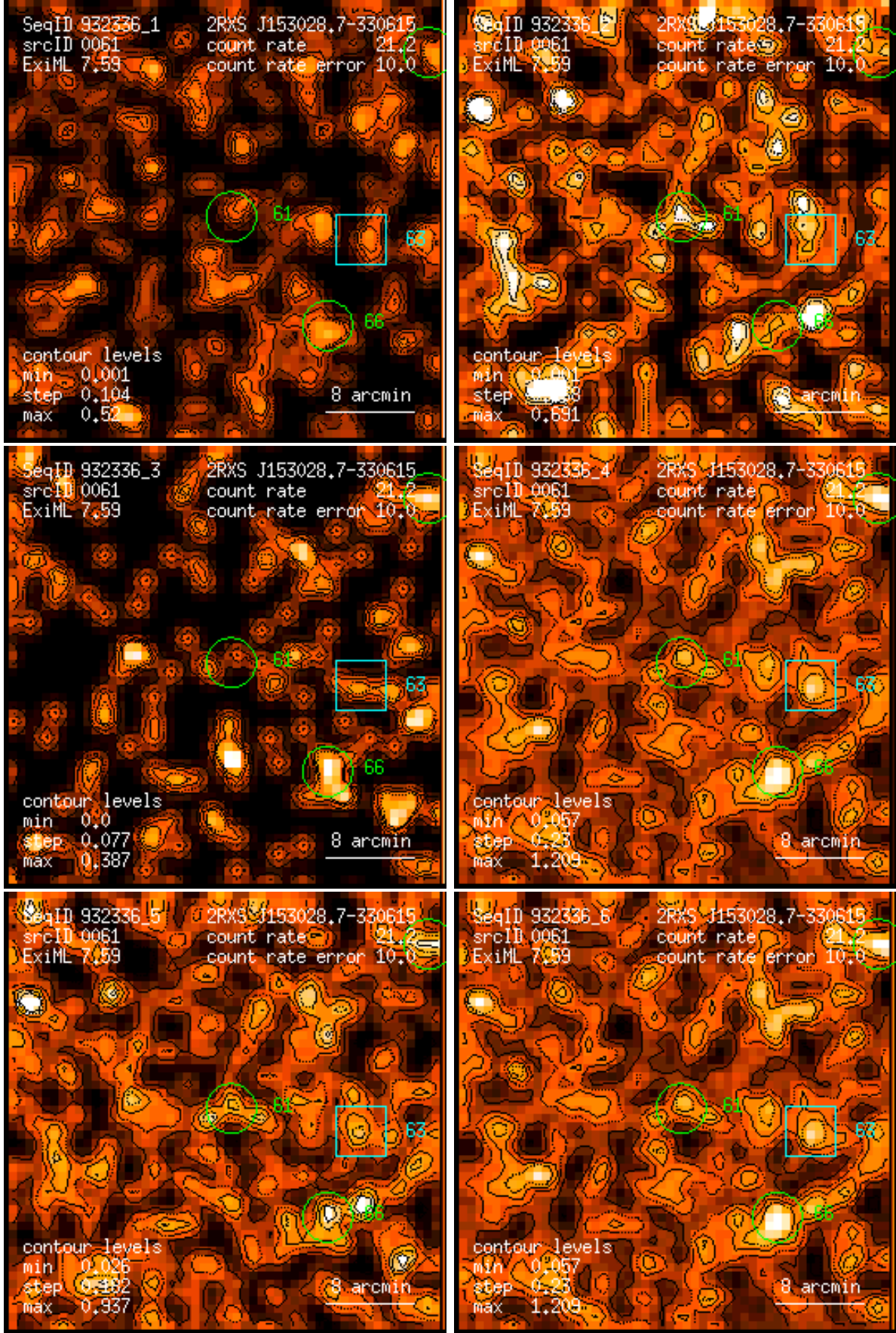
Figure 61: RASS 932336: detection 0061: band rate images, Gaussian filter: (1) PSPC channels 11 – 41, (2) 52 – 90, (3) 91 – 201, (4) 11 – 235, (5) 52 – 201, (6) 11 – 201. Broad band rates in counts/ks. Band rate contour levels in counts/ks/arcmin 2 .
