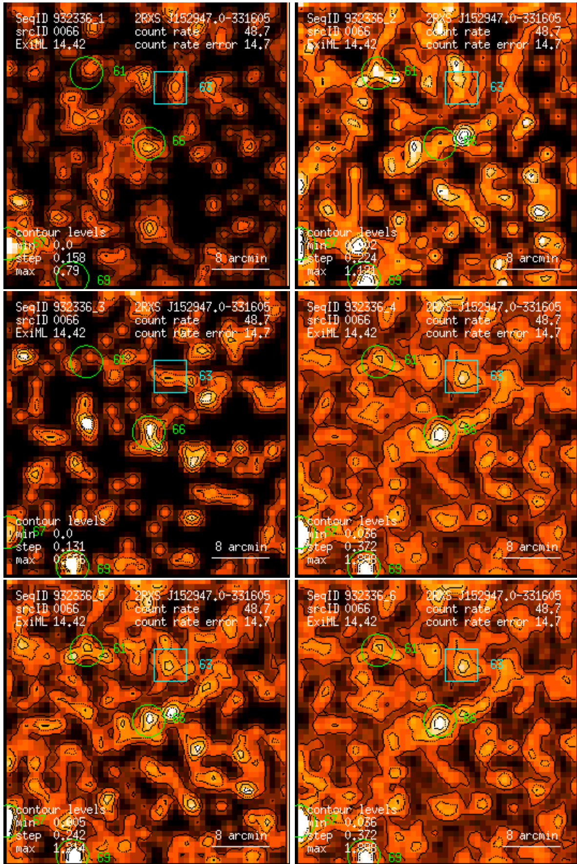
Figure 66: RASS 932336: detection 0066: band rate images, Gaussian filter: (1) PSPC channels 11 – 41, (2) 52 – 90, (3) 91 – 201, (4) 11 – 235, (5) 52 – 201, (6) 11 – 201. Broad band rates in counts/ks. Band rate contour levels in counts/ks/arcmin 2 .
