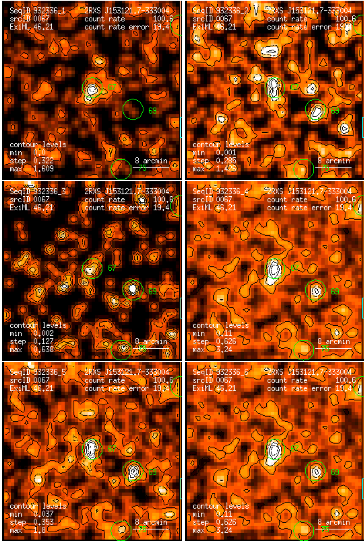
Figure 67: RASS 932336: detection 0067: band rate images, Gaussian filter: (1) PSPC channels 11 – 41, (2) 52 – 90, (3) 91 – 201, (4) 11 – 235, (5) 52 – 201, (6) 11 – 201. Broad band rates in counts/ks. Band rate contour levels in counts/ks/arcmin 2 .
