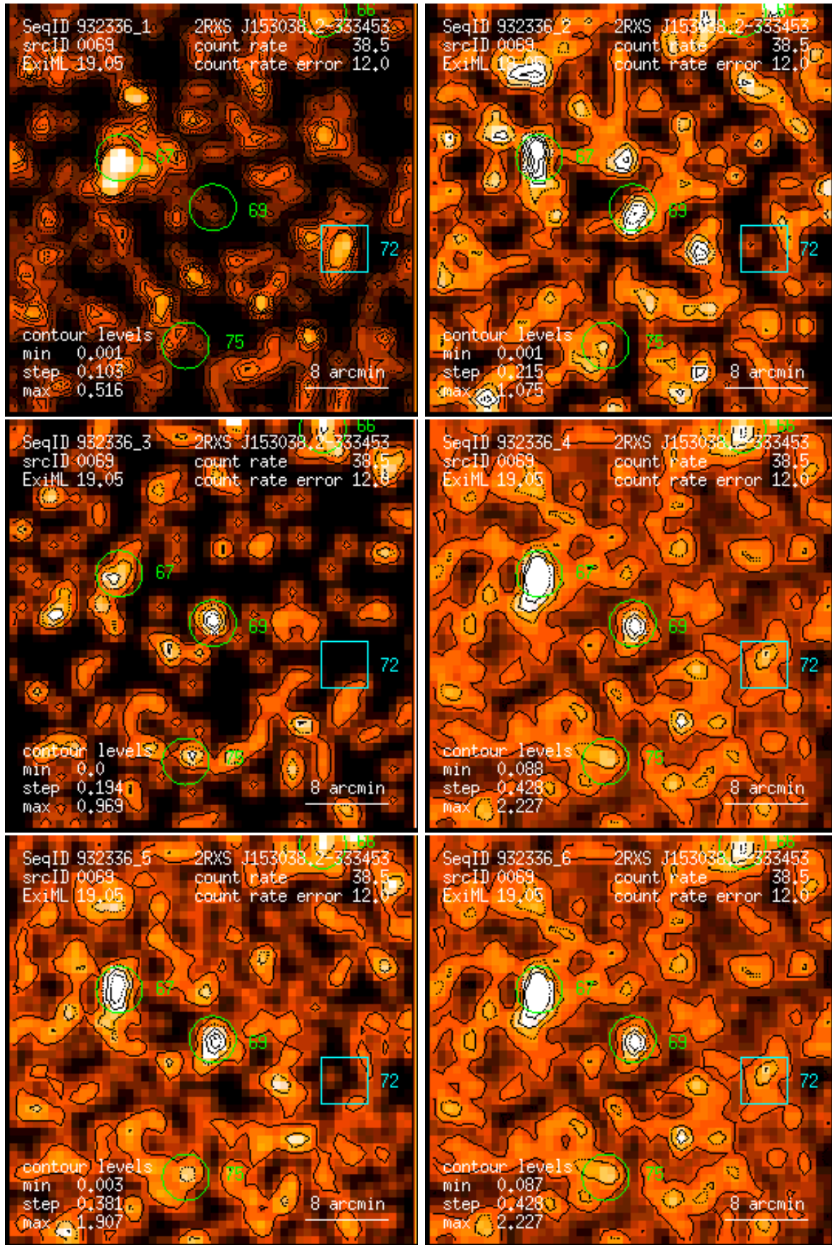
Figure 69: RASS 932336: detection 0069: band rate images, Gaussian filter: (1) PSPC channels 11 – 41, (2) 52 – 90, (3) 91 – 201, (4) 11 – 235, (5) 52 – 201, (6) 11 – 201. Broad band rates in counts/ks. Band rate contour levels in counts/ks/arcmin 2 .
