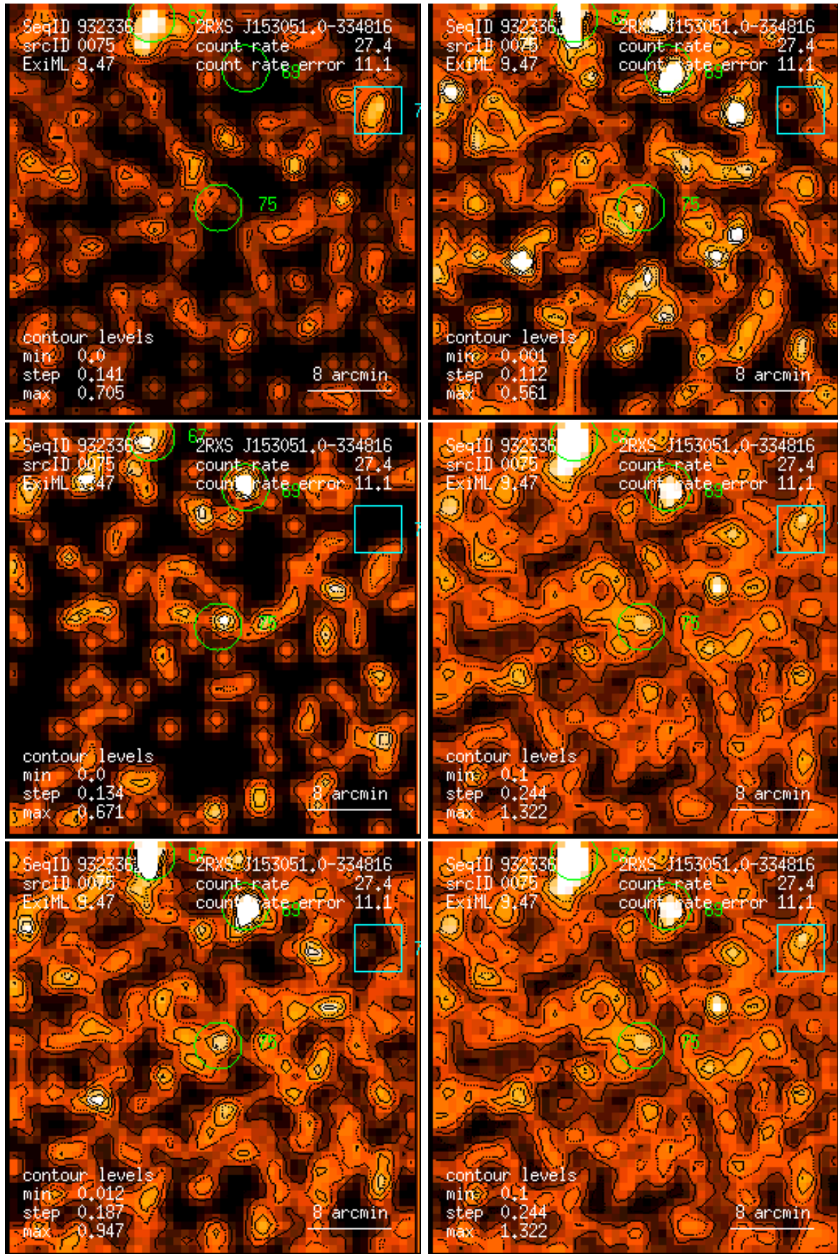
Figure 75: RASS 932336: detection 0075: band rate images, Gaussian filter: (1) PSPC channels 11 – 41, (2) 52 – 90, (3) 91 – 201, (4) 11 – 235, (5) 52 – 201, (6) 11 – 201. Broad band rates in counts/ks. Band rate contour levels in counts/ks/arcmin 2 .
