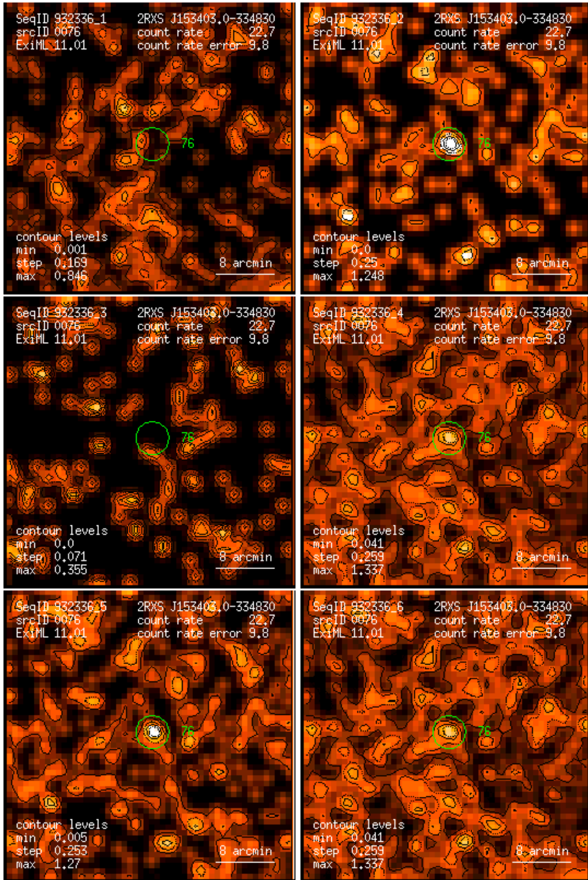
Figure 76: RASS 932336: detection 0076: band rate images, Gaussian filter: (1) PSPC channels 11 – 41, (2) 52 – 90, (3) 91 – 201, (4) 11 – 235, (5) 52 – 201, (6) 11 – 201. Broad band rates in counts/ks. Band rate contour levels in counts/ks/arcmin 2 .
