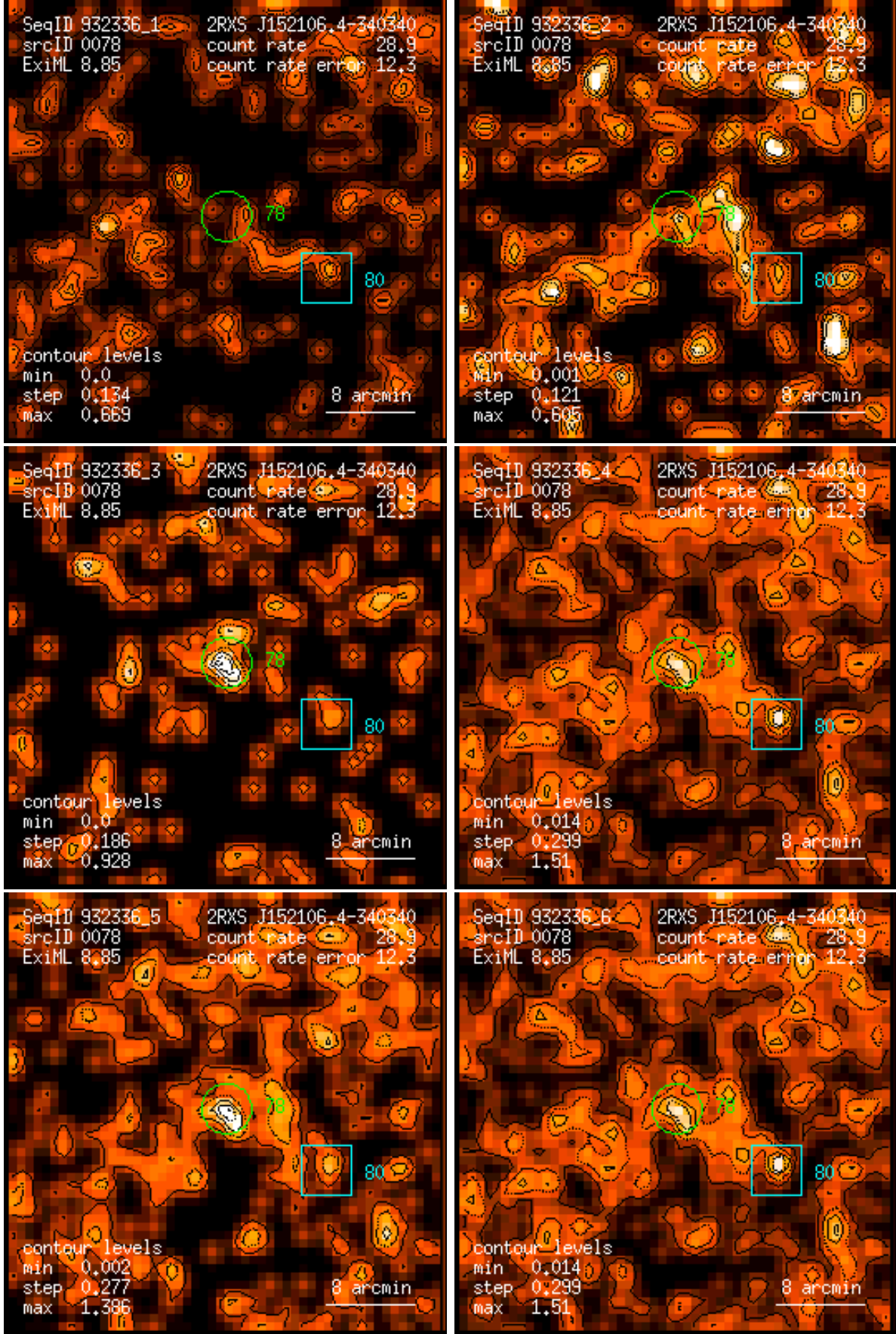
Figure 78: RASS 932336: detection 0078: band rate images, Gaussian filter: (1) PSPC channels 11 – 41, (2) 52 – 90, (3) 91 – 201, (4) 11 – 235, (5) 52 – 201, (6) 11 – 201. Broad band rates in counts/ks. Band rate contour levels in counts/ks/arcmin 2 .
