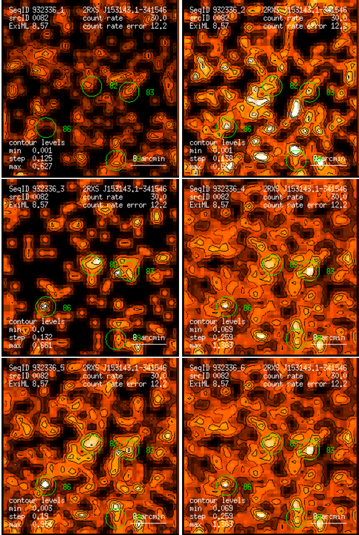
Figure 82: RASS 932336: detection 0082: band rate images, Gaussian filter: (1) PSPC channels 11 – 41, (2) 52 – 90, (3) 91 – 201, (4) 11 – 235, (5) 52 – 201, (6) 11 – 201. Broad band rates in counts/ks. Band rate contour levels in counts/ks/arcmin 2 .
