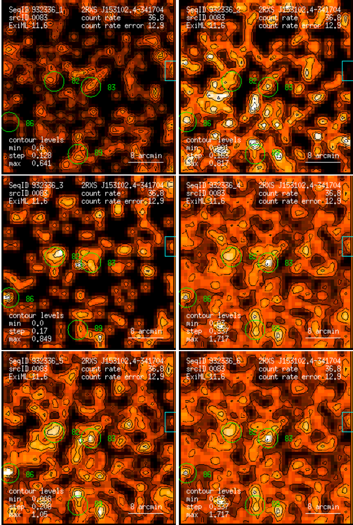
Figure 83: RASS 932336: detection 0083: band rate images, Gaussian filter: (1) PSPC channels 11 – 41, (2) 52 – 90, (3) 91 – 201, (4) 11 – 235, (5) 52 – 201, (6) 11 – 201. Broad band rates in counts/ks. Band rate contour levels in counts/ks/arcmin 2 .
