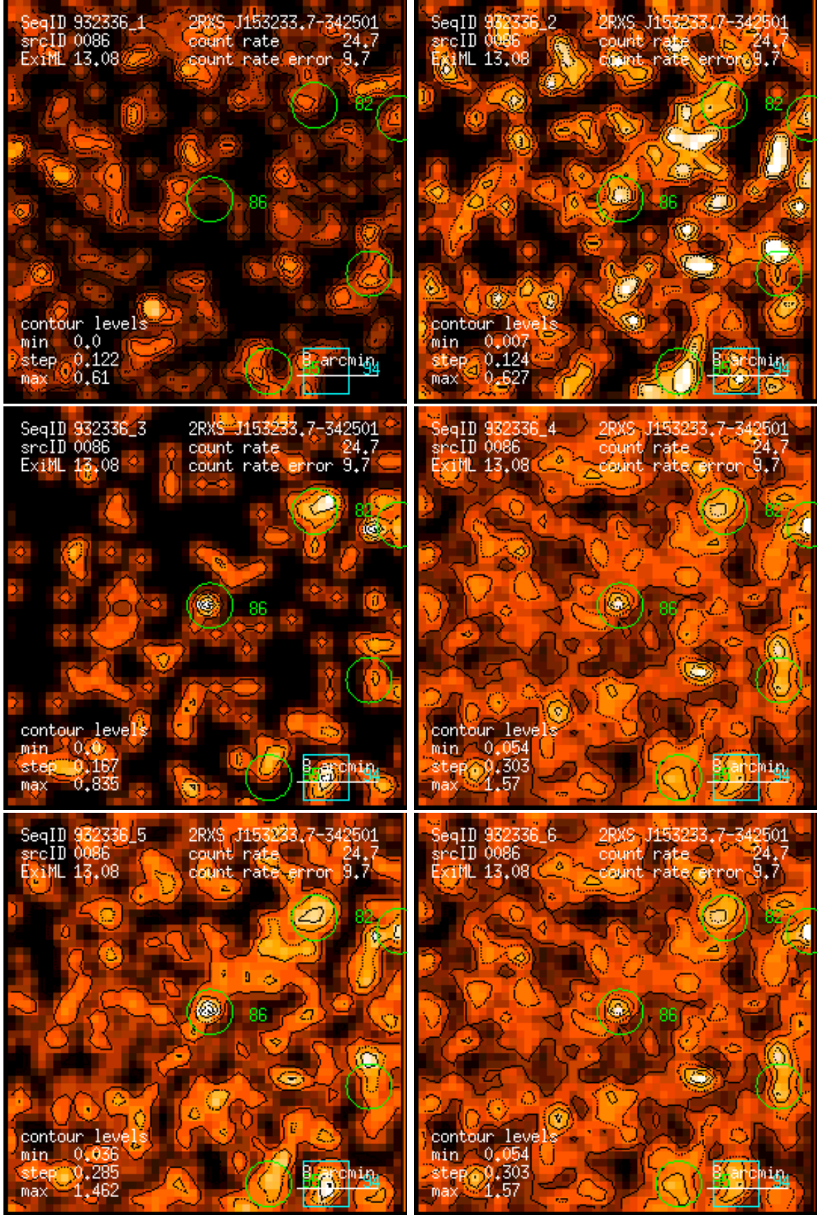
Figure 86: RASS 932336: detection 0086: band rate images, Gaussian filter: (1) PSPC channels 11 – 41, (2) 52 – 90, (3) 91 – 201, (4) 11 – 235, (5) 52 – 201, (6) 11 – 201. Broad band rates in counts/ks. Band rate contour levels in counts/ks/arcmin 2 .
