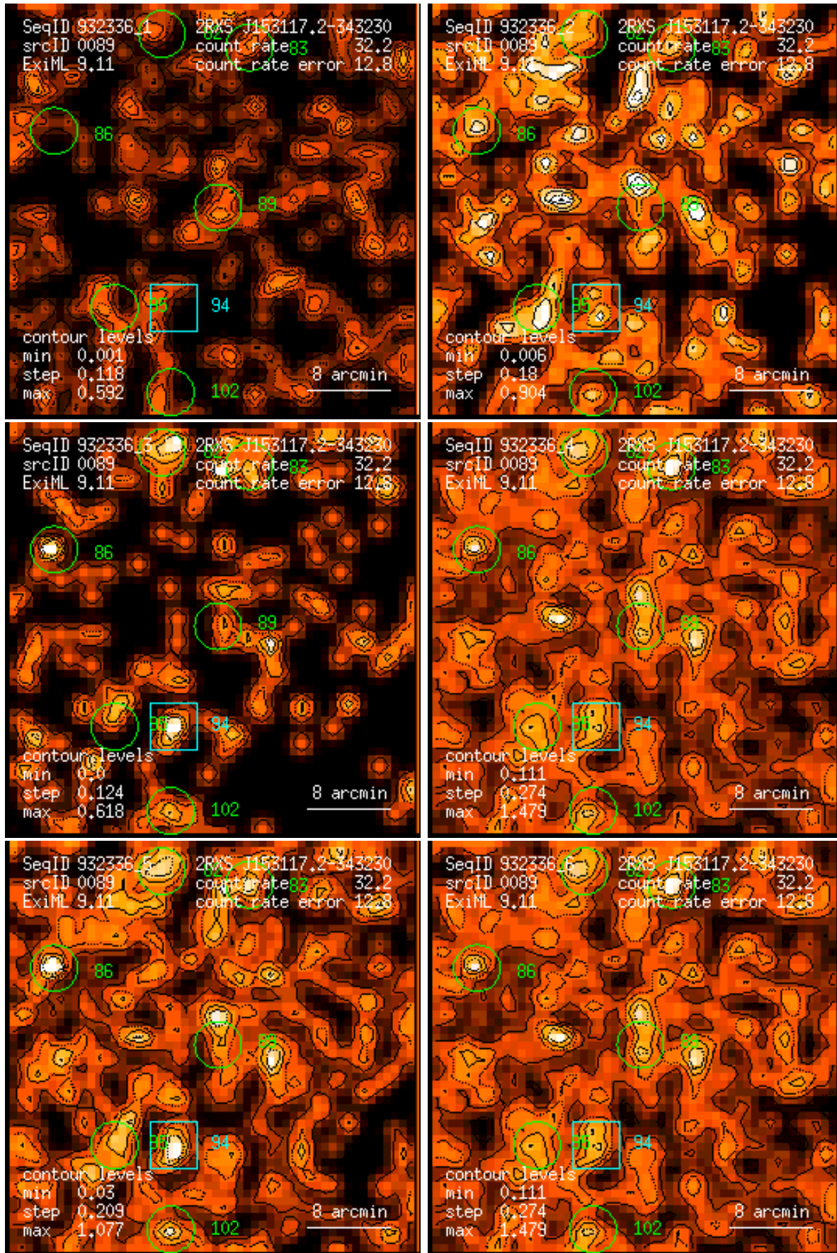
Figure 89: RASS 932336: detection 0089: band rate images, Gaussian filter: (1) PSPC channels 11 – 41, (2) 52 – 90, (3) 91 – 201, (4) 11 – 235, (5) 52 – 201, (6) 11 – 201. Broad band rates in counts/ks. Band rate contour levels in counts/ks/arcmin 2 .
