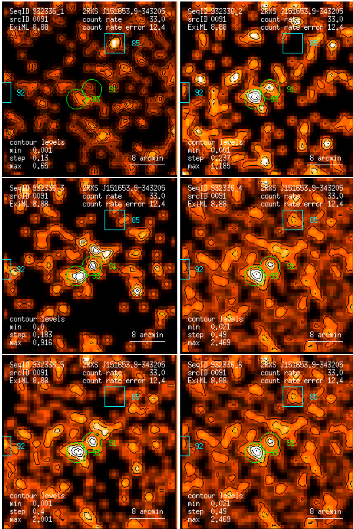
Figure 91: RASS 932336: detection 0091: band rate images, Gaussian filter: (1) PSPC channels 11 – 41, (2) 52 – 90, (3) 91 – 201, (4) 11 – 235, (5) 52 – 201, (6) 11 – 201. Broad band rates in counts/ks. Band rate contour levels in counts/ks/arcmin 2 .
