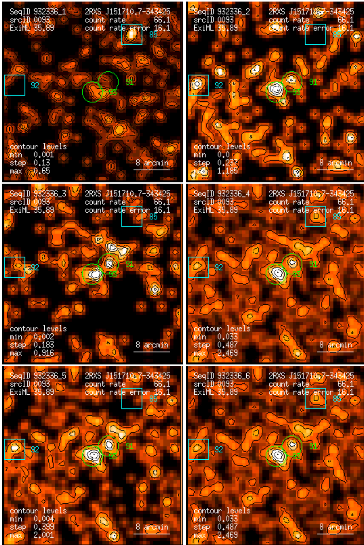
Figure 93: RASS 932336: detection 0093: band rate images, Gaussian filter: (1) PSPC channels 11 – 41, (2) 52 – 90, (3) 91 – 201, (4) 11 – 235, (5) 52 – 201, (6) 11 – 201. Broad band rates in counts/ks. Band rate contour levels in counts/ks/arcmin 2 .
