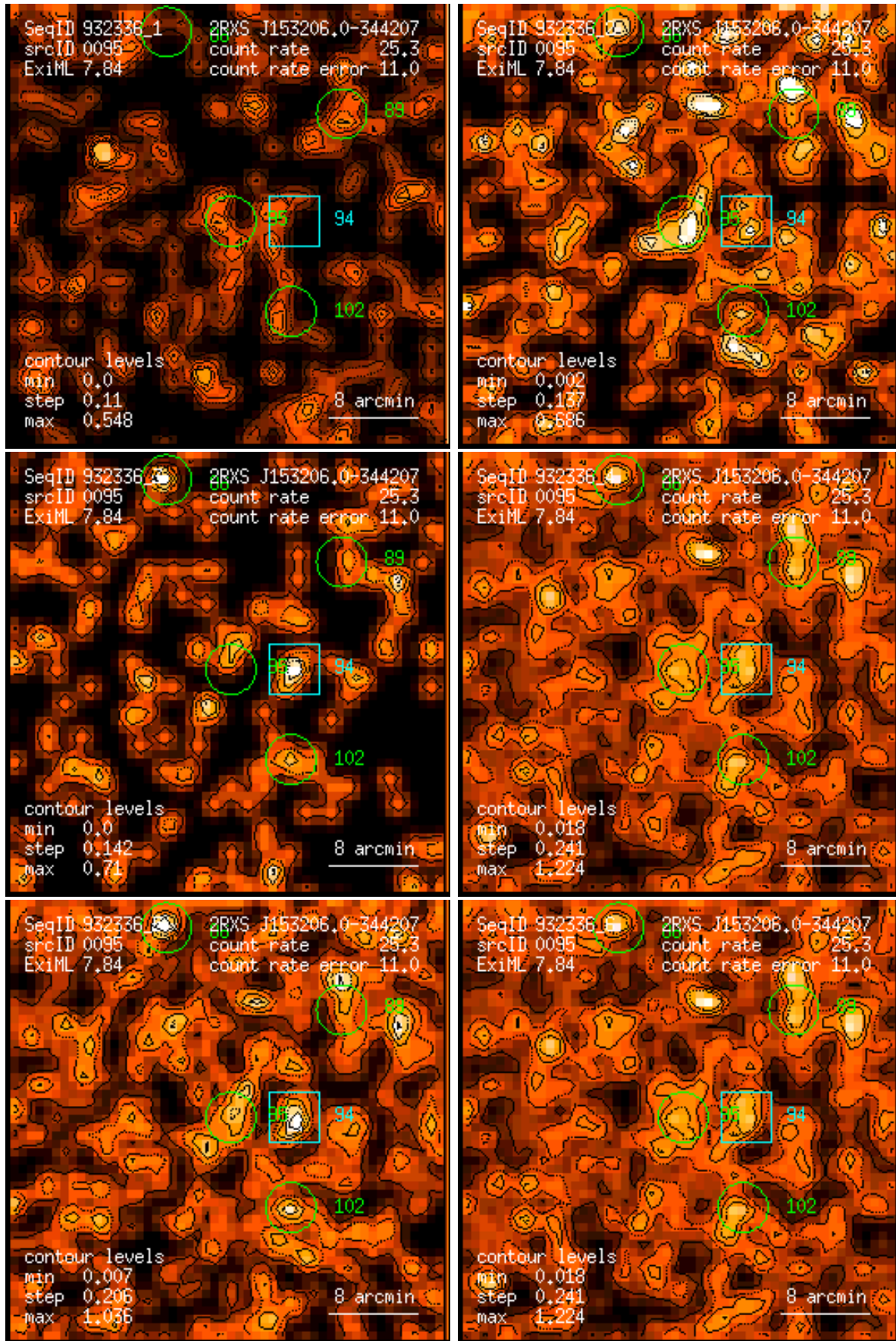
Figure 95: RASS 932336: detection 0095: band rate images, Gaussian filter: (1) PSPC channels 11 – 41, (2) 52 – 90, (3) 91 – 201, (4) 11 – 235, (5) 52 – 201, (6) 11 – 201. Broad band rates in counts/ks. Band rate contour levels in counts/ks/arcmin 2 .
