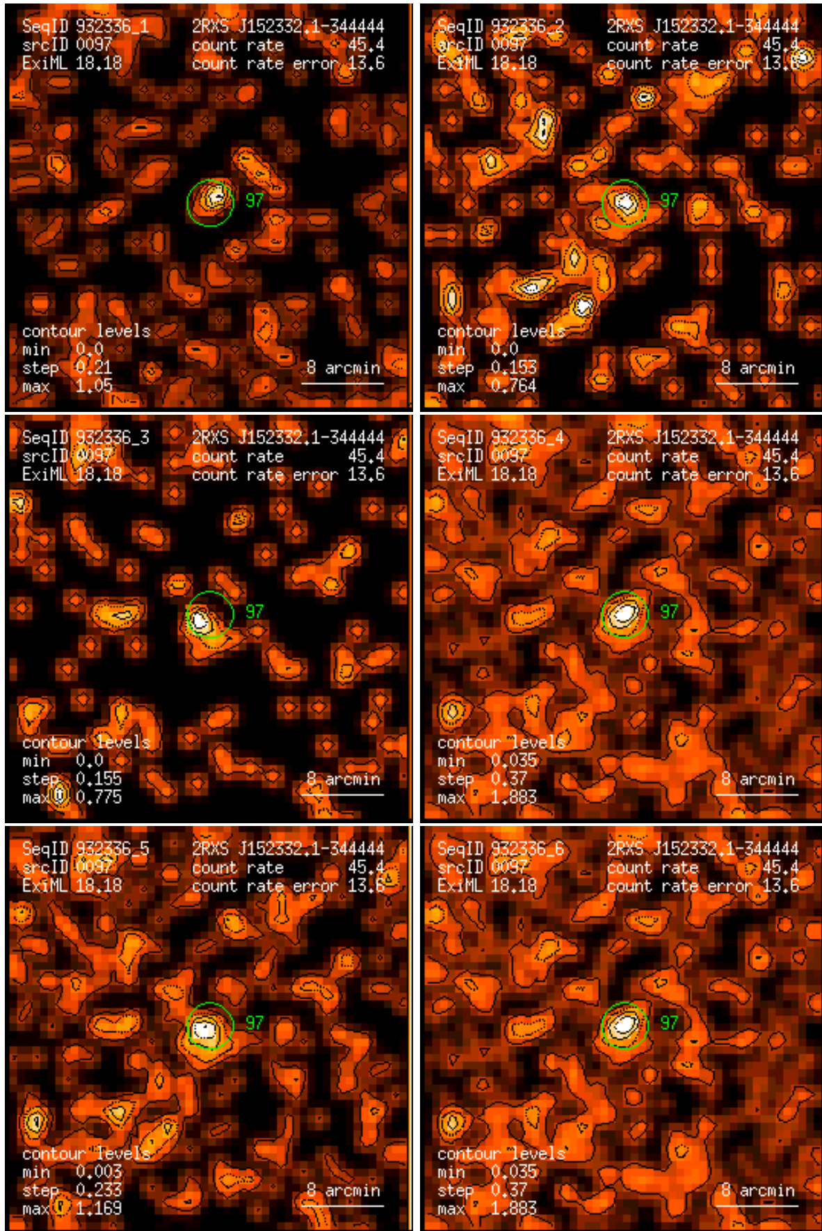
Figure 97: RASS 932336: detection 0097: band rate images, Gaussian filter: (1) PSPC channels 11 – 41, (2) 52 – 90, (3) 91 – 201, (4) 11 – 235, (5) 52 – 201, (6) 11 – 201. Broad band rates in counts/ks. Band rate contour levels in counts/ks/arcmin 2 .
